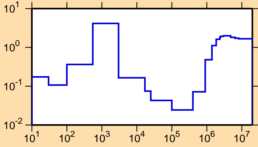
\sigma vs. E for ^{82}\text{As}(n,\text{nonel.})
