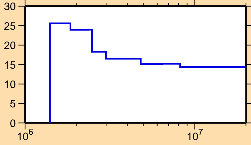
\Delta\sigma/\sigma vs. E for ^{82}\text{As}(n,n\text{onel.})
