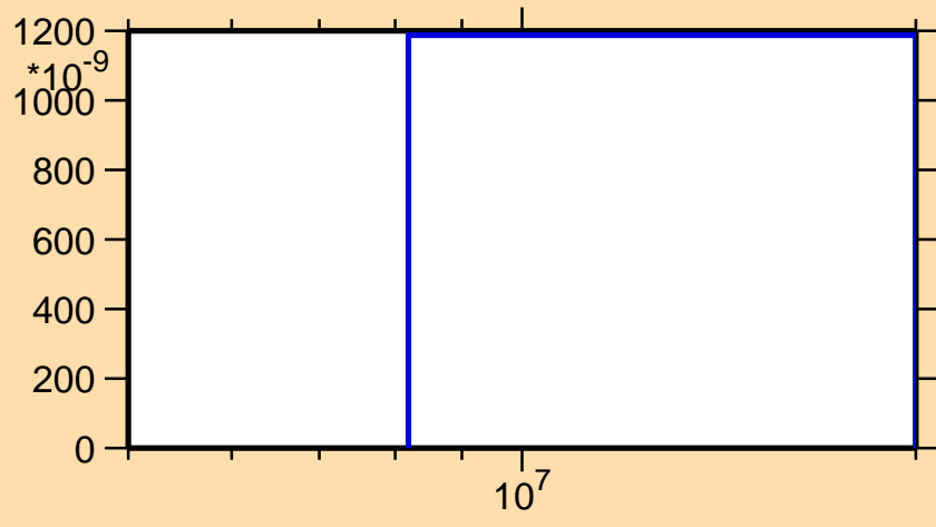
\sigma vs. E for ^{82}\text{As}(n,n\alpha)
