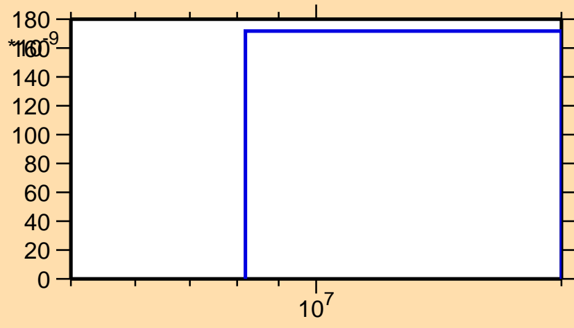
\sigma vs. E for ^{82}\text{As}(n,nd)
