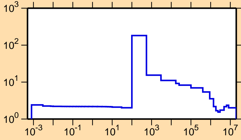
\sigma vs. E for ^{82}\text{As}(n,\text{el.})
