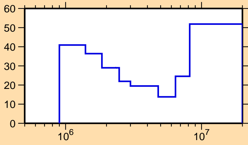
\Delta\sigma/\sigma vs. E for ^{82}\text{As}(n,ncont.)
