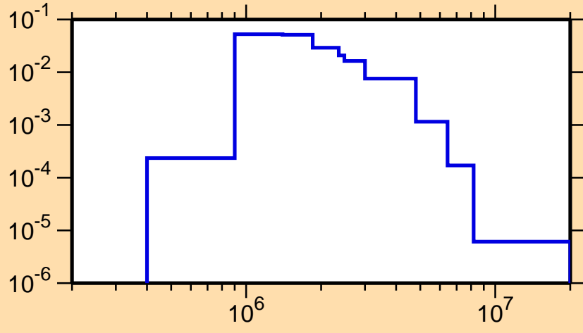
\sigma vs. E for ^{82}\text{As}(n,n_3)
