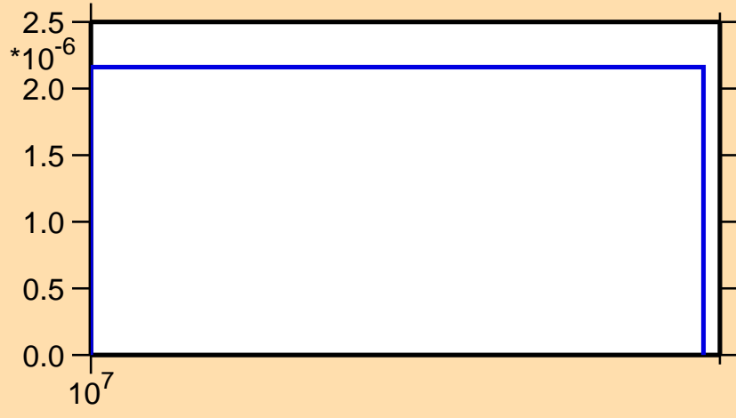
\sigma vs. E for ^{83}\text{As}(n,t)
