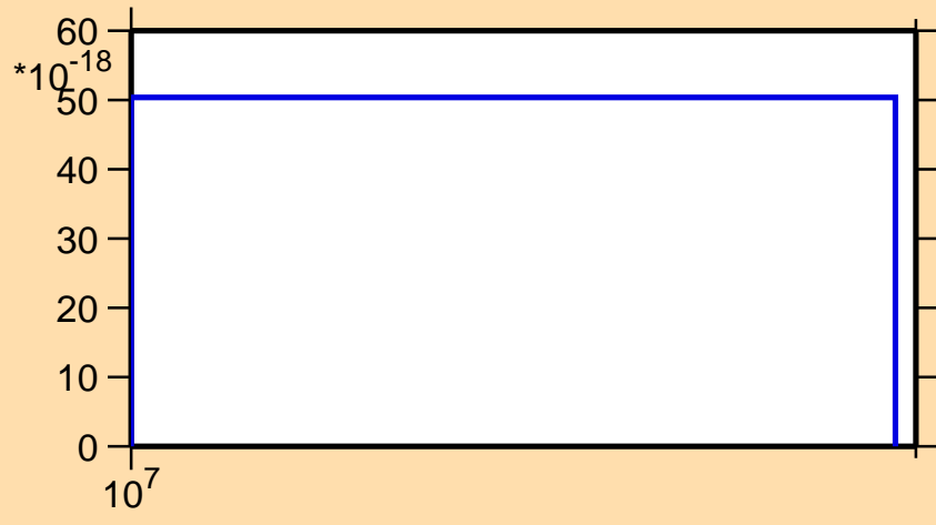
\sigma vs. E for ^{83}\text{As}(n,2np)
