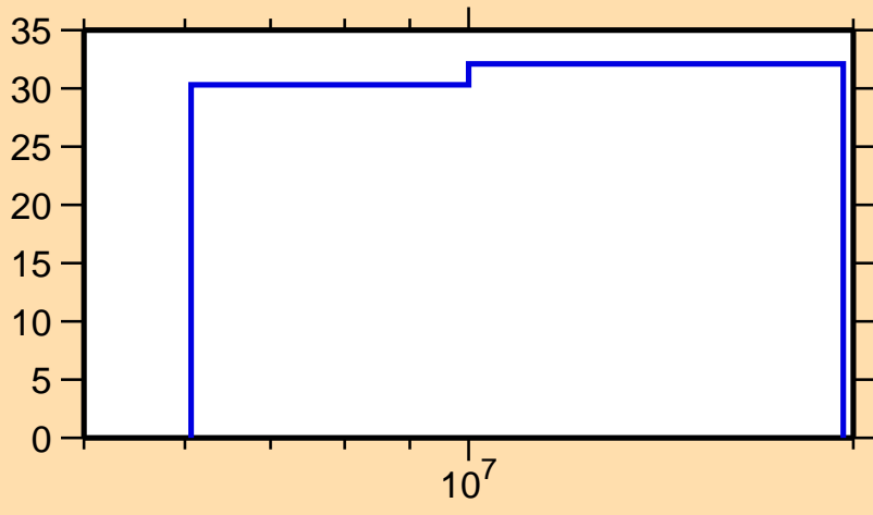
\Delta\sigma/\sigma vs. E for ^{83}\text{As}(n,ncont.)
