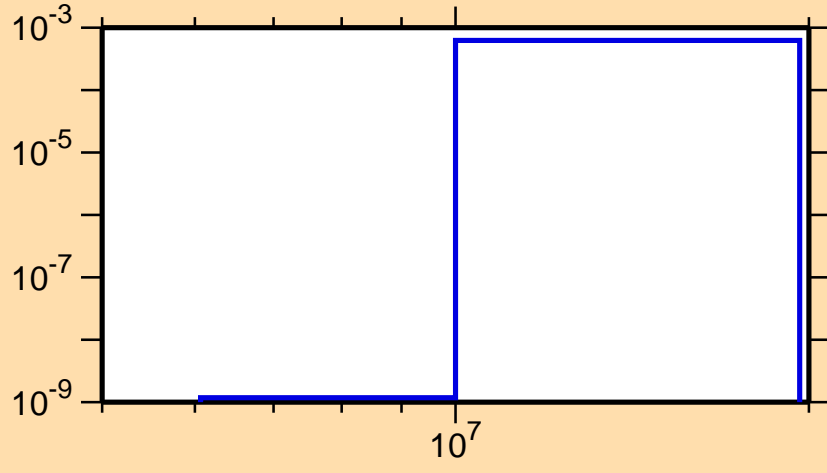
\sigma vs. E for ^{83}\text{As}(n,p)
