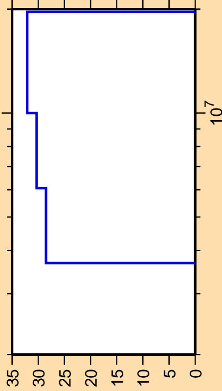
\Delta\sigma/\sigma vs. E for ^{83}\text{As}(n,n\text{cont.})
