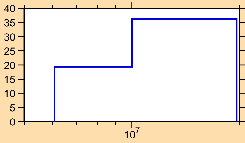
\Delta\sigma/\sigma vs. E for ^{83}\text{As}(n,el.)
