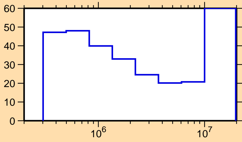
\Delta\sigma/\sigma vs. E for ^{83}\text{As}(n,\text{inel.})
