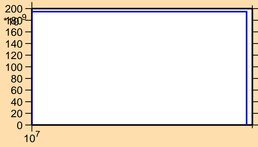
\sigma vs. E for ^{83}\text{As}(n,n\alpha)
