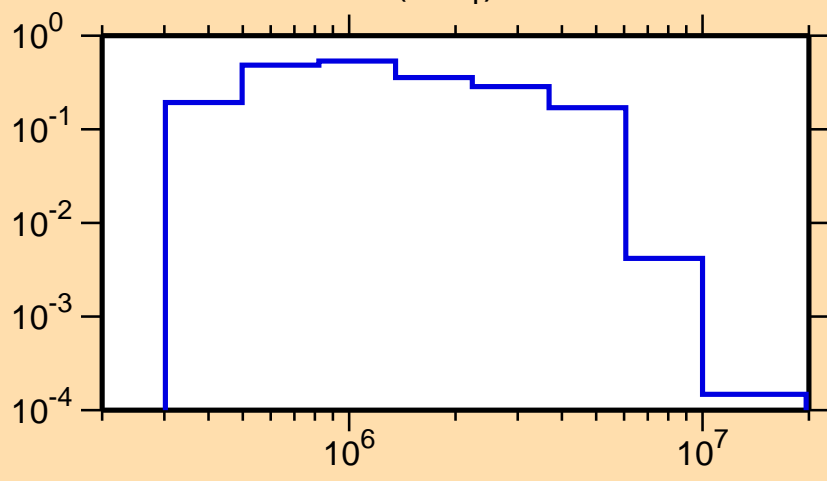
\sigma vs. E for ^{83}\text{As}(n,n_1)
