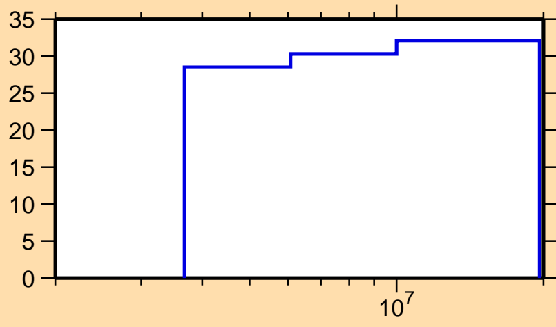
\Delta\sigma/\sigma vs. E for ^{83}\text{As}(n,n\text{cont.})
