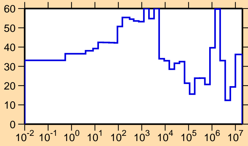
\Delta\sigma/\sigma vs. E for ^{83}\text{As}(n,\text{el.})
