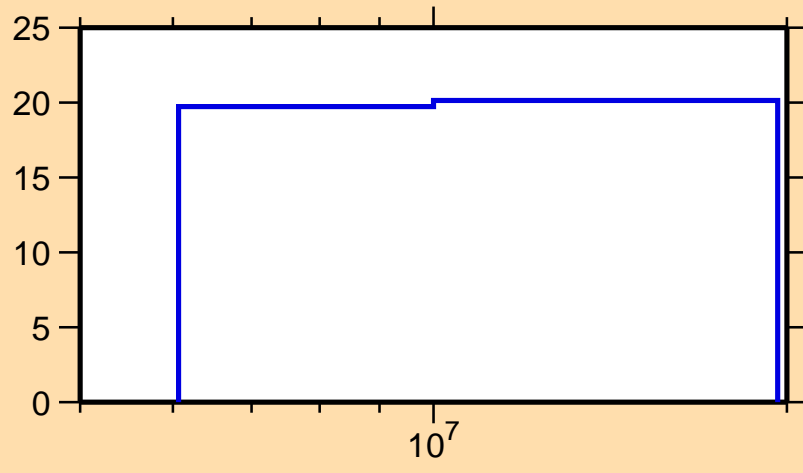
\Delta\sigma/\sigma vs. E for ^{83}\text{As}(n,\text{nonel.})
