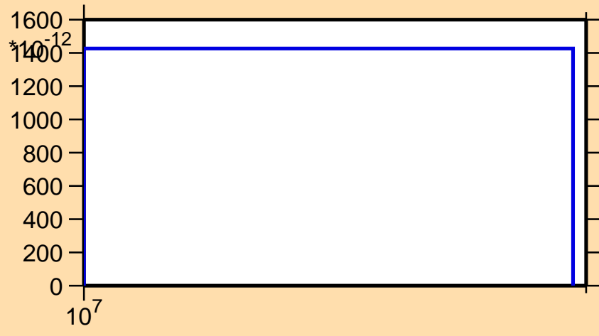
\sigma vs. E for ^{83}\text{As}(n,nt)
