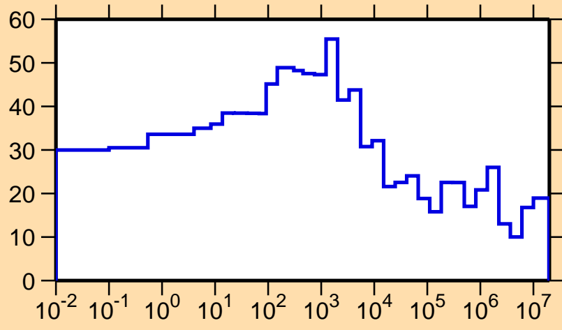
\Delta\sigma/\sigma vs. E for ^{83}\text{As}(n,\text{tot.})
