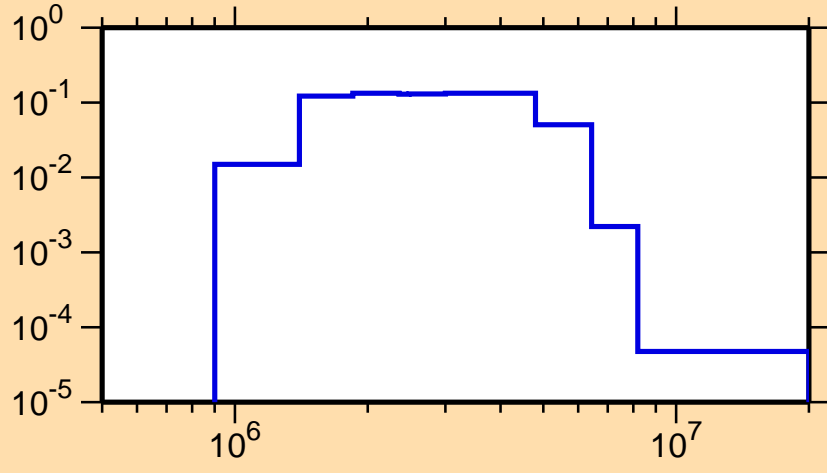
\sigma vs. E for ^{83}\text{As}(n,n_4)
