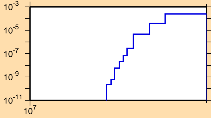
\sigma vs. E for ^{85}\text{As}(n,np)
