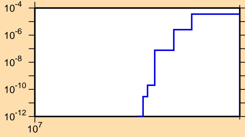
\sigma vs. E for ^{85}\text{As}(n,nt)
