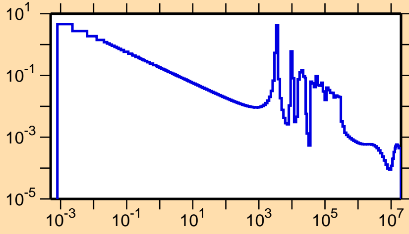
\sigma vs. E for ^{85}\text{As}(n,\gamma)
