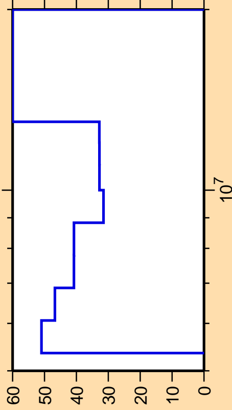
\Delta\sigma/\sigma vs. E for ^{85}\text{As}(n,2n)
