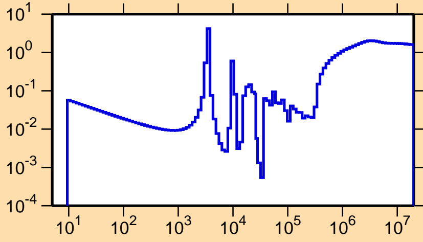
\sigma vs. E for ^{85}\text{As}(n,\text{nonel.})
