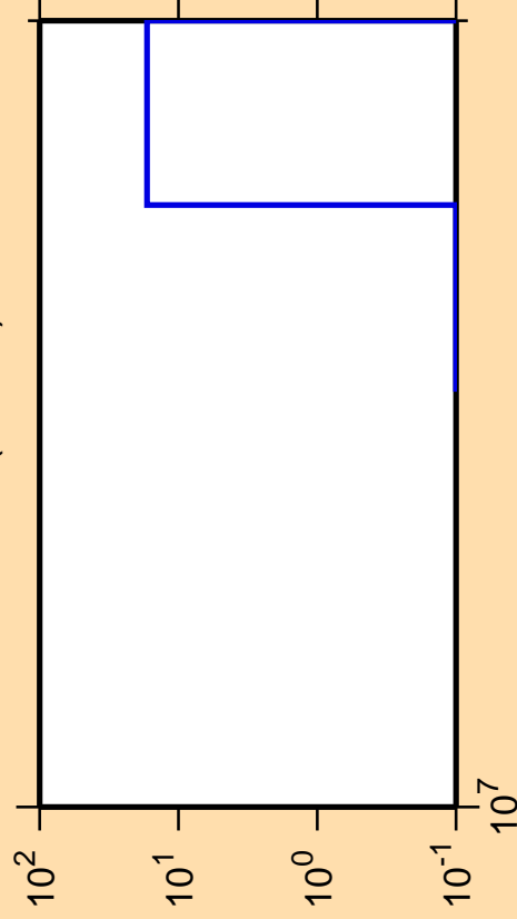
\Delta\sigma/\sigma vs. E for ^{85}\text{As}(n,2n\alpha)
