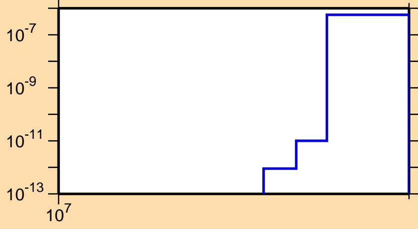
\sigma vs. E for ^{85}\text{As}(n,\text{nd})
