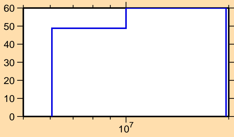
\Delta\sigma/\sigma vs. E for ^{85}\text{As}(n,n_1)
