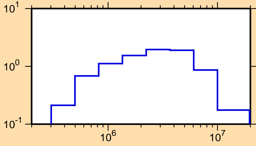
\sigma vs. E for ^{85}\text{As}(n,\text{inel.})
