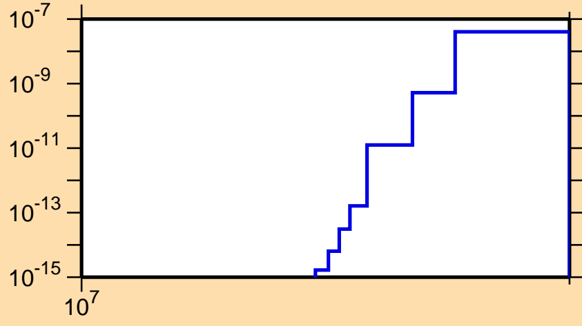
\sigma vs. E for ^{197}\text{At}(n,nt)
