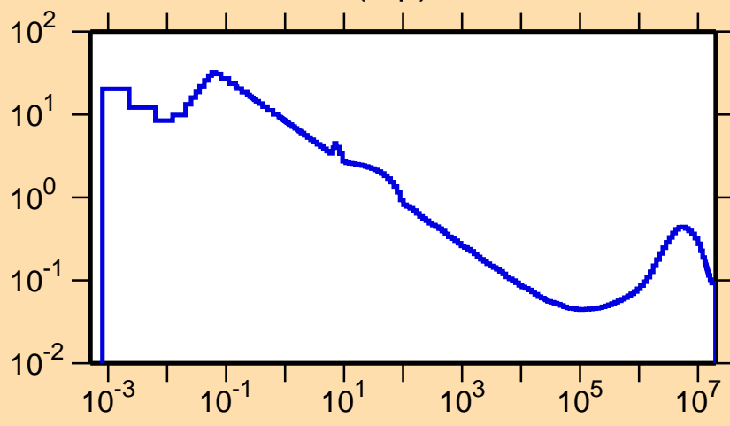
\sigma vs. E for ^{197}\text{At}(n,p)
