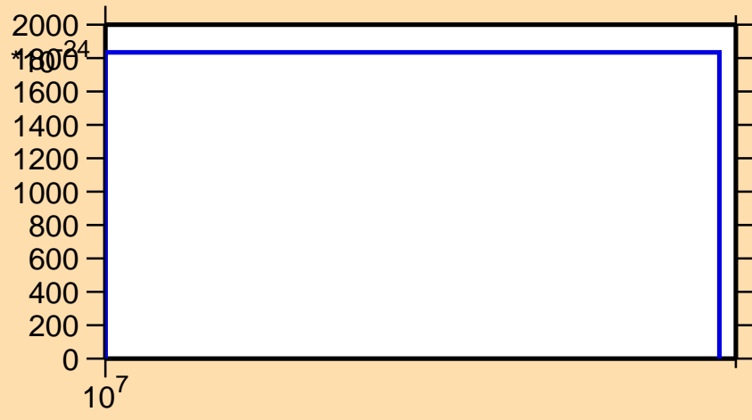
\sigma vs. E for ^{197}\text{At}(\text{mt } 42)
