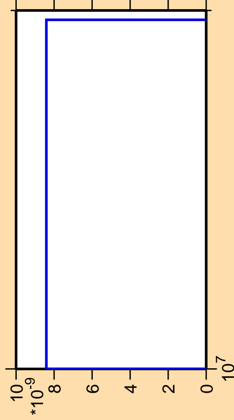
\Delta\sigma/\sigma vs. E for ^{197}\text{At}(\text{mt } 42)
