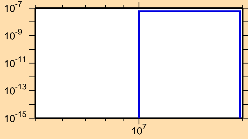
\sigma vs. E for ^{197}\text{At}(n,\text{nd})
