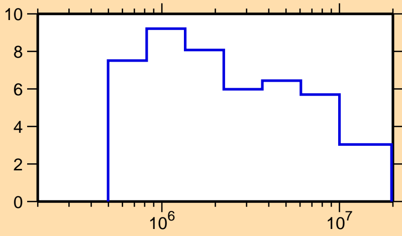
\Delta\sigma/\sigma vs. E for ^{197}\text{At}(n,\text{tot.})
