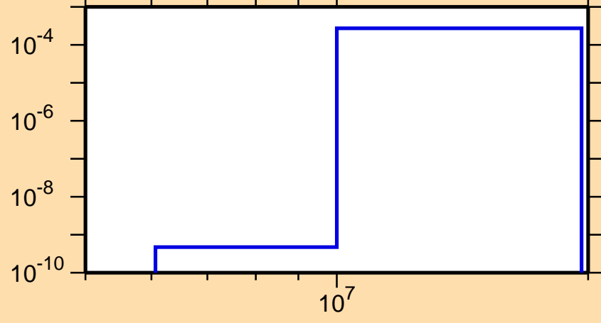
\sigma vs. E for ^{197}\text{At}(n,t)
