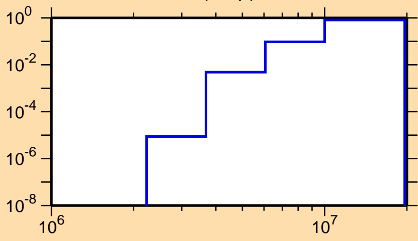
\sigma vs. E for ^{197}\text{At}(n,np)
