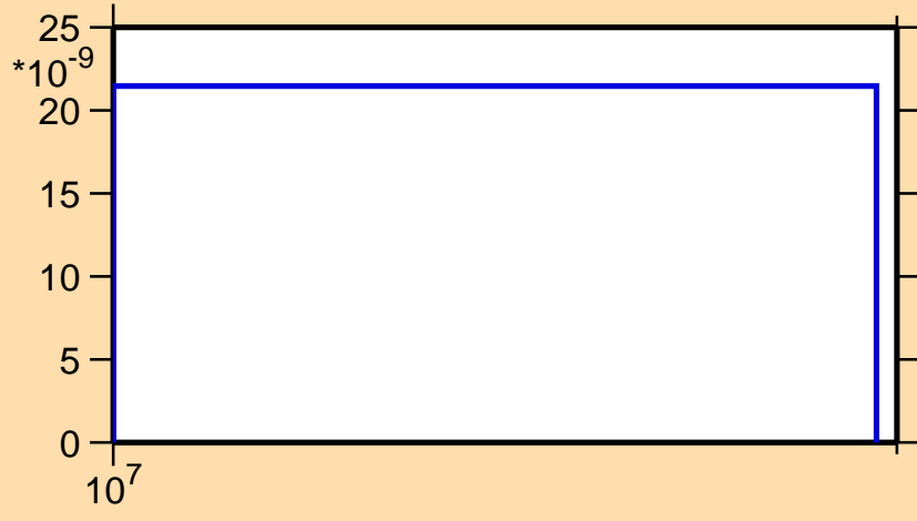
\sigma vs. E for ^{197}\text{At}(n,3n)
