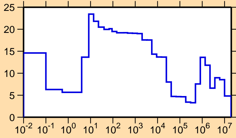
\Delta\sigma/\sigma vs. E for ^{197}\text{At}(n,\text{el.})
