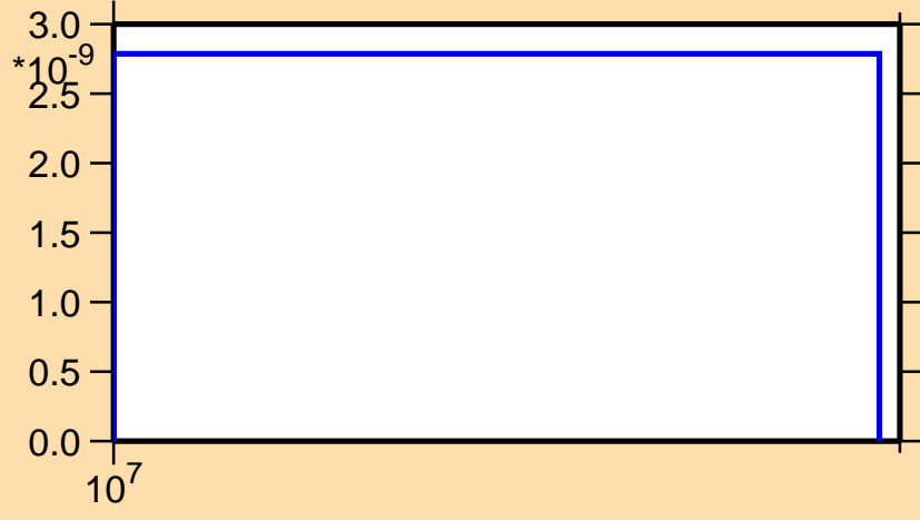
\sigma vs. E for ^{197}\text{At}(n,3n\alpha)
