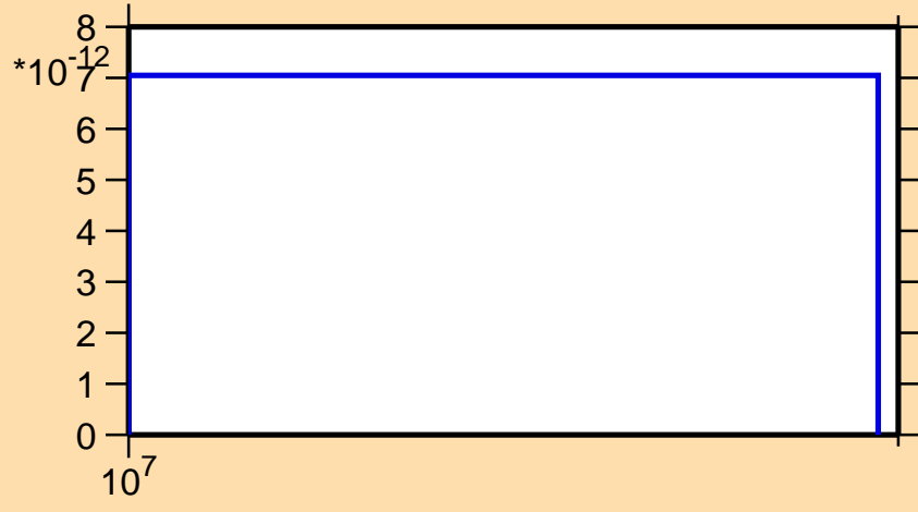
\sigma vs. E for ^{197}\text{At}(\text{mt } 34)
