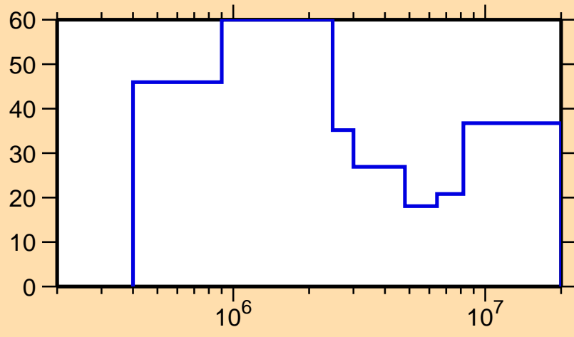
\Delta\sigma/\sigma vs. E for ^{197}\text{At}(n,n\text{cont.})
