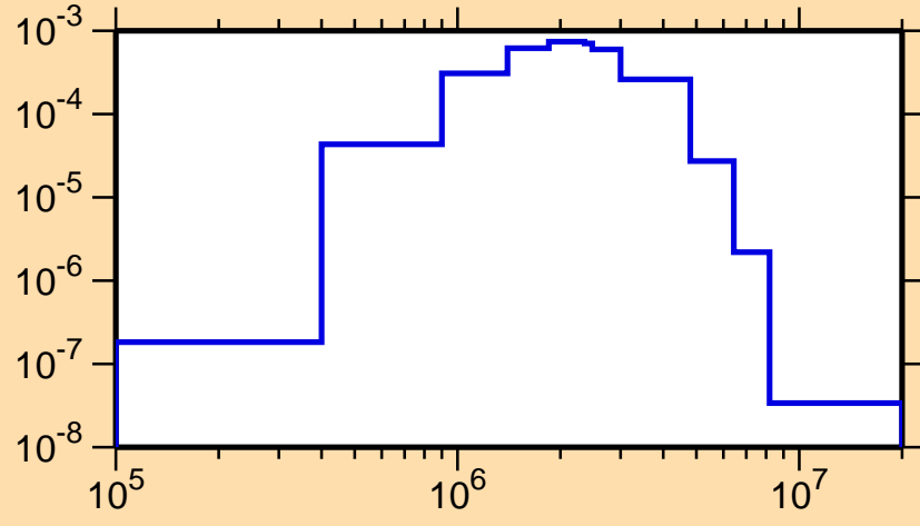
\sigma vs. E for ^{197}\text{At}(n,n_3)
