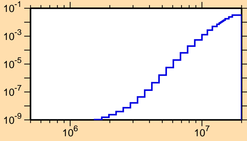
\sigma vs. E for ^{198}\text{At}(n,n\alpha)
