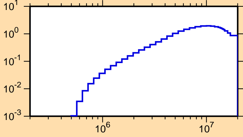
\sigma vs. E for ^{198}\text{At}(n,n\text{cont.})
