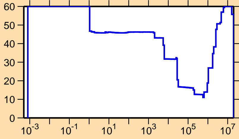
\Delta\sigma/\sigma vs. E for ^{198}\text{At}(n,\gamma)
