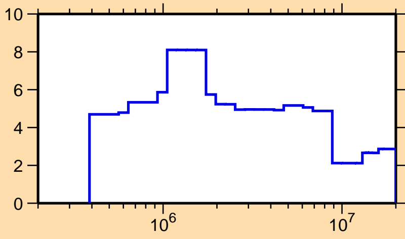
\Delta\sigma/\sigma vs. E for ^{198}\text{At}(n,\text{tot.})
