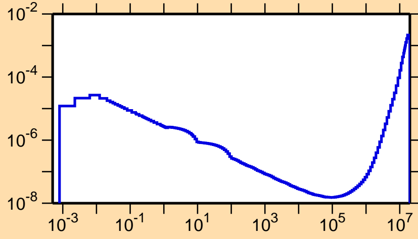
\sigma vs. E for ^{198}\text{At}(n,p\alpha)
