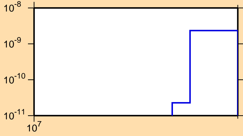
\sigma vs. E for ^{198}\text{At}(n,nt)
