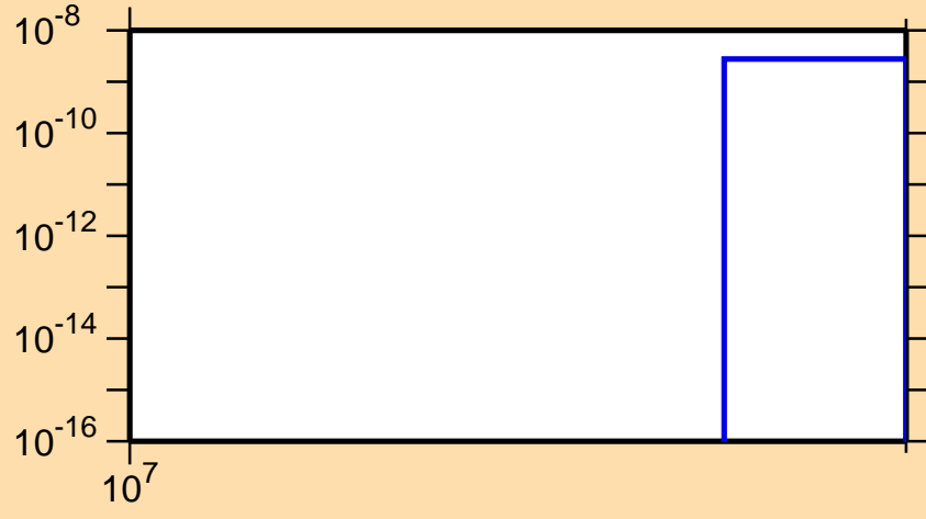
\sigma vs. E for ^{198}\text{At}(n,3n\alpha)
