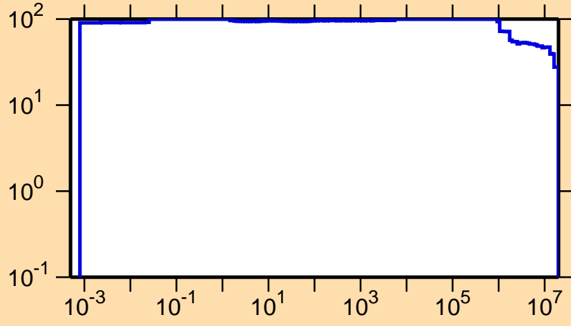
\Delta\sigma/\sigma vs. E for ^{198}\text{At}(n,p)
