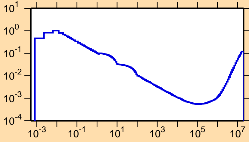
\sigma vs. E for ^{198}\text{At}(n,\alpha)
