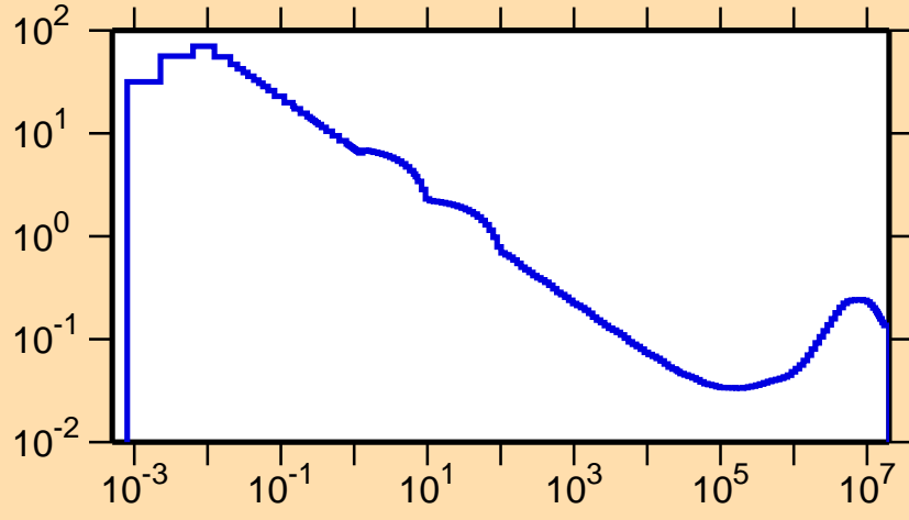
\sigma vs. E for ^{198}\text{At}(n,p)
