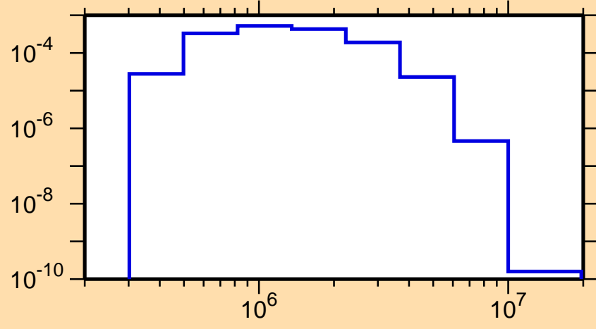
\sigma vs. E for ^{198}\text{At}(n,n_4)
