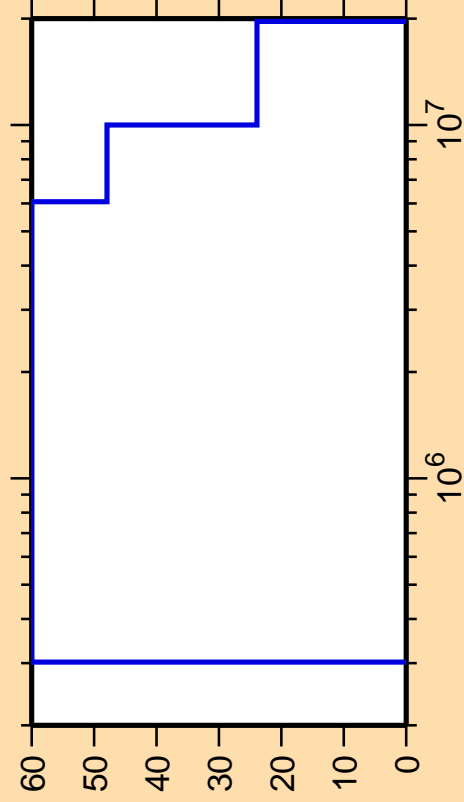
\Delta\sigma/\sigma vs. E for ^{198}\text{At}(n,n_4)
