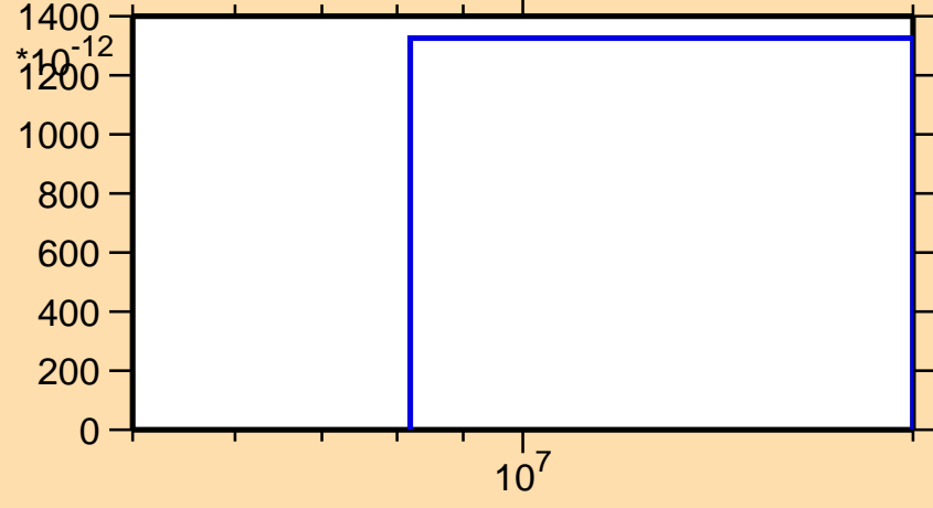
\sigma vs. E for ^{198}\text{At}(n,\text{pt})
