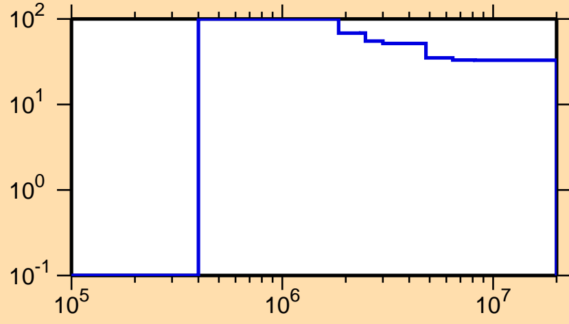
\Delta\sigma/\sigma vs. E for ^{198}\text{At}(n,n_1)
