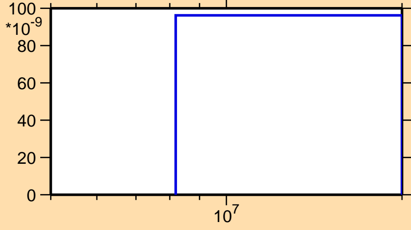
\sigma vs. E for ^{198}\text{At}(n,\text{pd})
