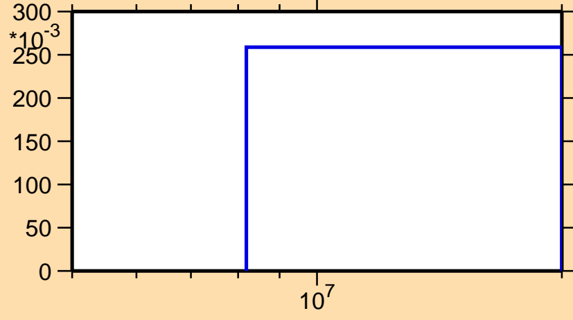
\sigma vs. E for ^{198}\text{At}(n,2n)
