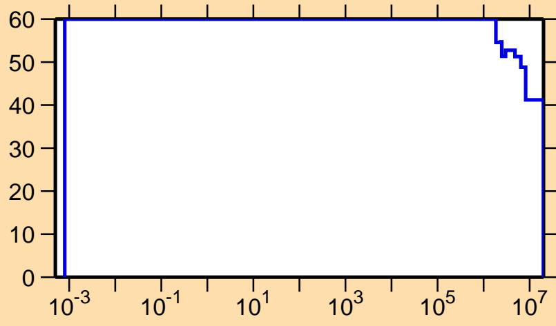
\Delta\sigma/\sigma vs. E for ^{198}\text{At}(n,p)
