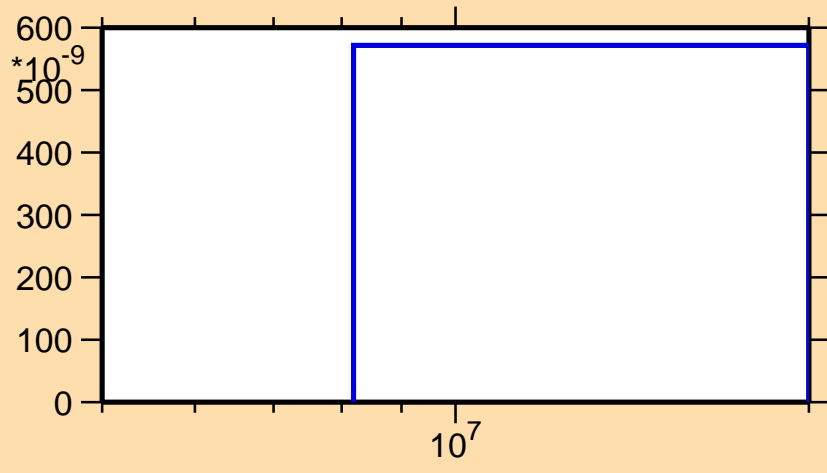
\sigma vs. E for ^{198}\text{At}(n,\text{nd})
