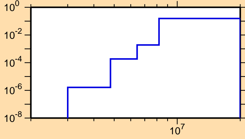
\sigma vs. E for ^{198}\text{At}(n,np)
