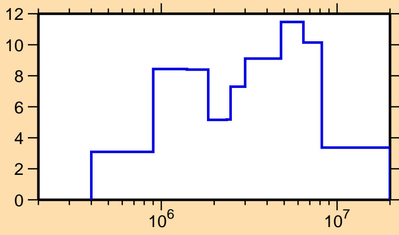
\Delta\sigma/\sigma vs. E for ^{198}\text{At}(n, el.)
