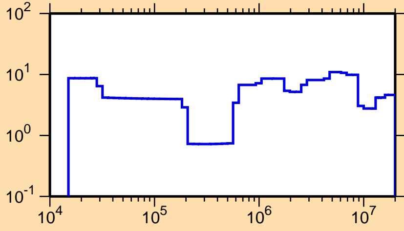
\Delta\sigma/\sigma vs. E for ^{198}\text{At}(n, el.)
