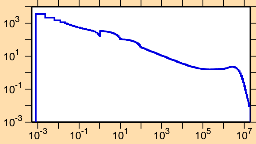
\sigma vs. E for ^{198}\text{At}(n,\gamma)
