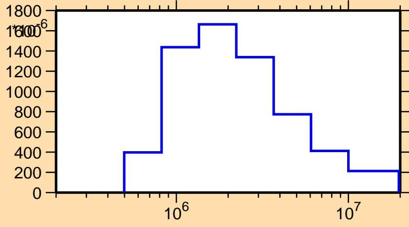
\sigma vs. E for ^{199}\text{At}(n,n_1)
