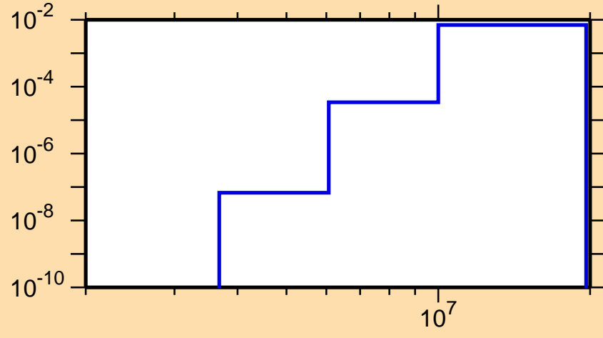
\sigma vs. E for ^{199}\text{At}(n,d)
