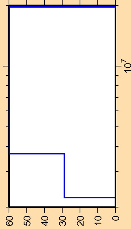
\Delta\sigma/\sigma vs. E for ^{199}\text{At}(n,d)
