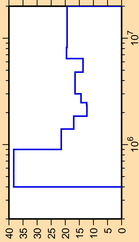
\Delta\sigma/\sigma vs. E for ^{199}\text{At}(n,n_3)
