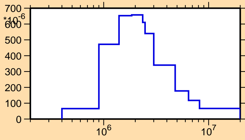
\sigma vs. E for ^{199}\text{At}(n,n_3)
