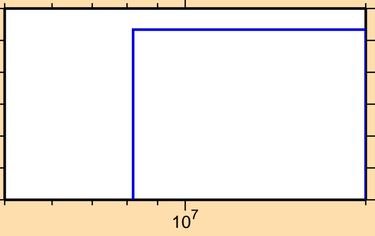
\sigma vs. E for ^{199}\text{At}(n,\text{pd})
