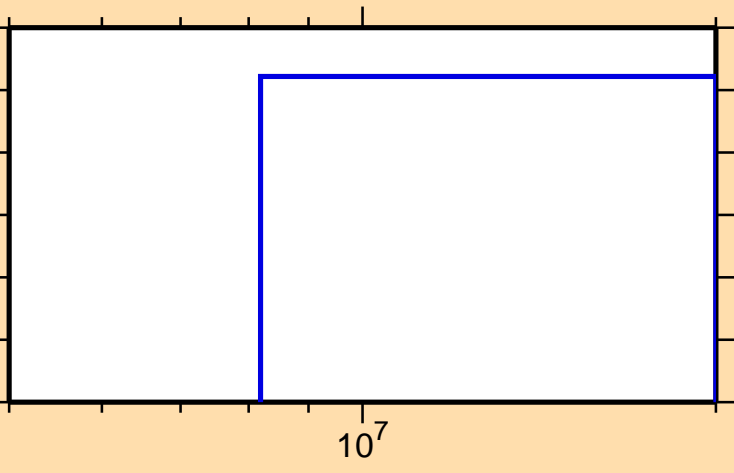
\sigma vs. E for ^{199}\text{At}(\text{mt } 34)
