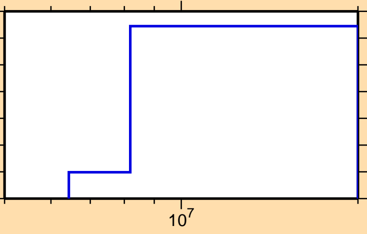
\sigma vs. E for ^{199}\text{At}(n,\text{He3})
