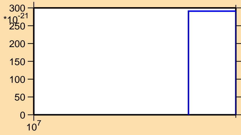
\sigma vs. E for ^{200}\text{At}(\text{mt } 42)
