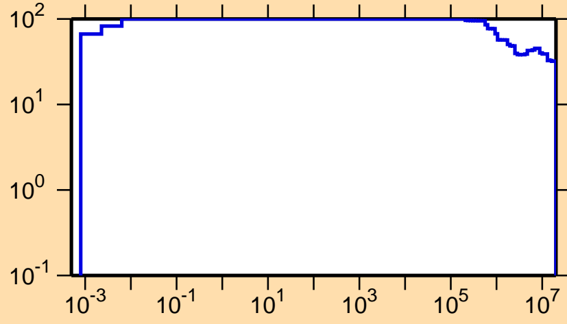
\Delta\sigma/\sigma vs. E for ^{200}\text{At}(n, p)
