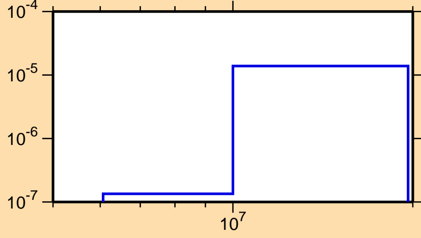
\sigma vs. E for ^{200}\text{At}(n,2n\alpha)
