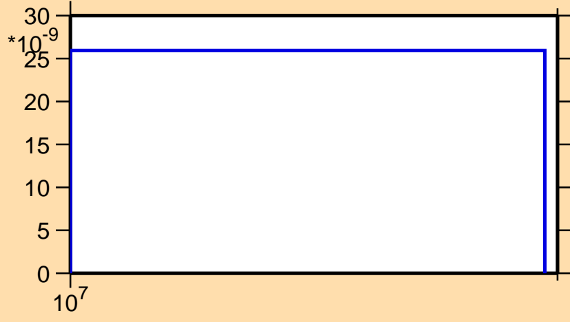
\sigma vs. E for ^{200}\text{At}(n,3n)
