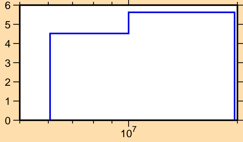
\Delta\sigma/\sigma vs. E for ^{200}\text{At}(n,\text{el.})
