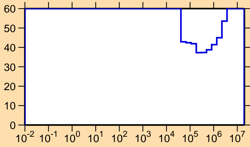
\Delta\sigma/\sigma vs. E for ^{200}\text{At}(n, \gamma)
