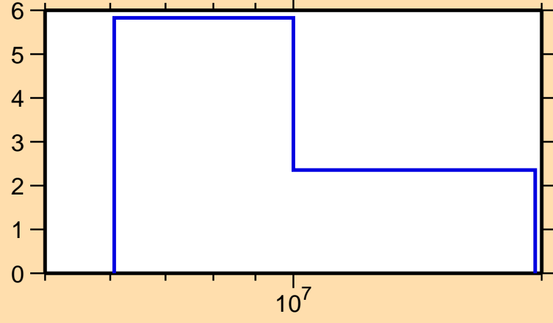
\Delta\sigma/\sigma vs. E for ^{200}\text{At}(n,\text{tot.})
