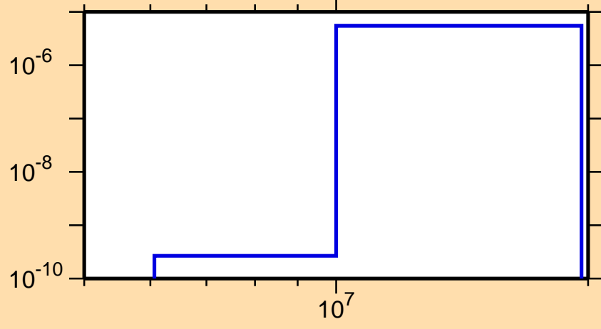
\sigma vs. E for ^{200}\text{At}(n,\text{He3})
