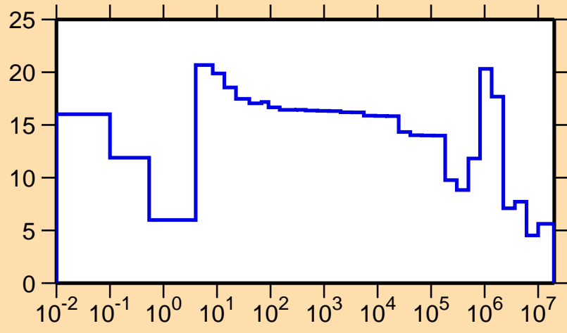
\Delta\sigma/\sigma vs. E for ^{200}\text{At}(n,\text{el.})
