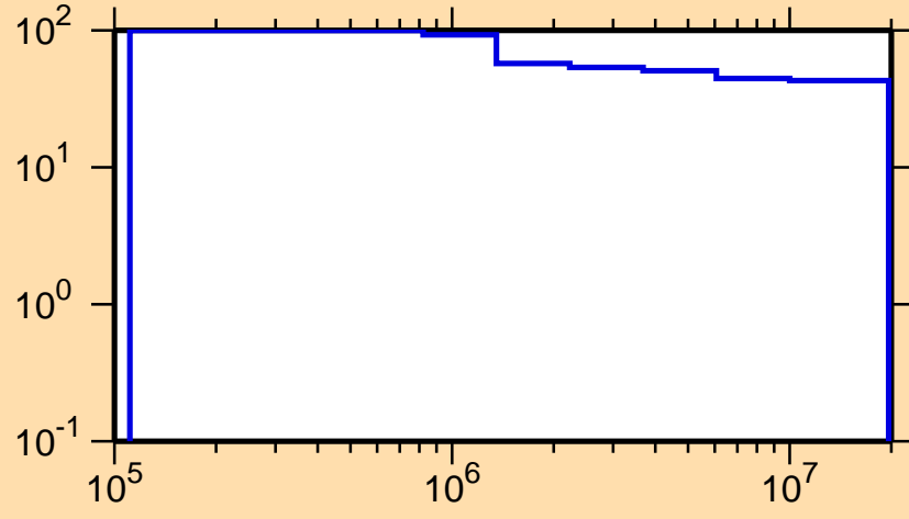
\Delta\sigma/\sigma vs. E for ^{200}\text{At}(n,n_1)
