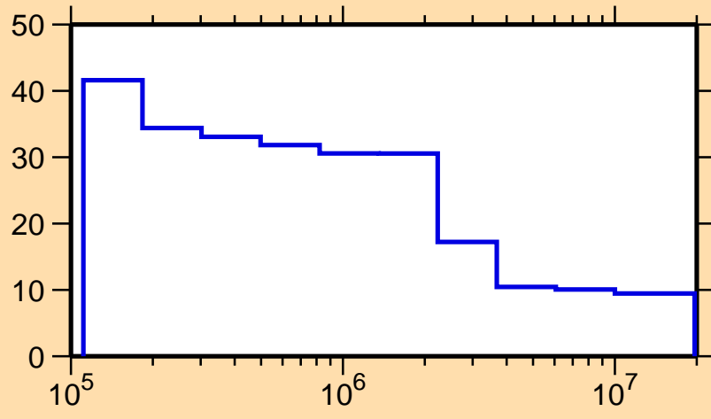
\Delta\sigma/\sigma vs. E for ^{200}\text{At}(n,\text{nonel.})
