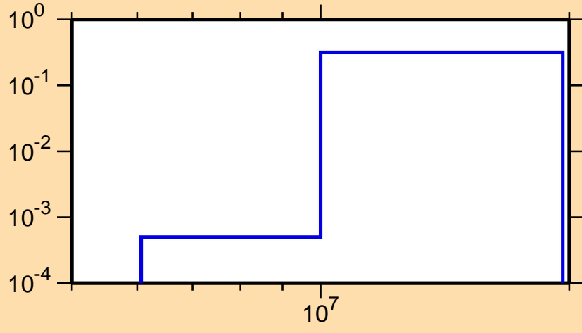
\sigma vs. E for ^{200}\text{At}(n,2n)
