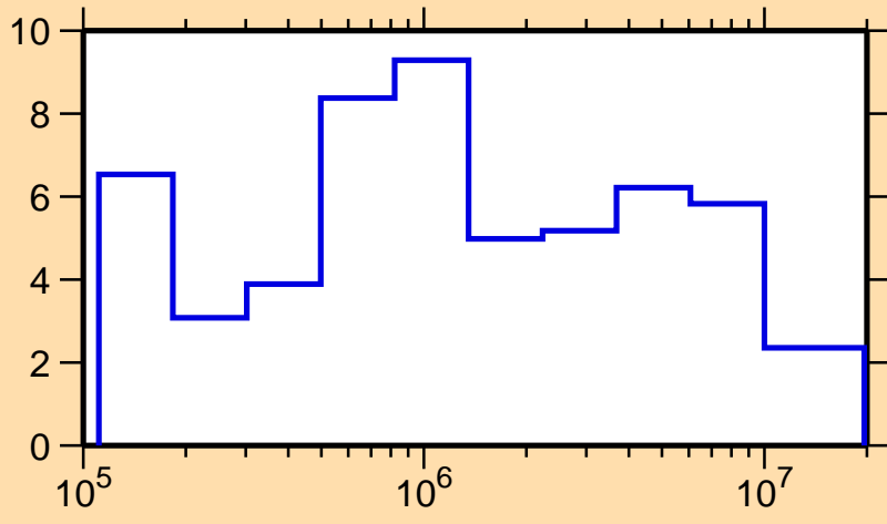
\Delta\sigma/\sigma vs. E for ^{200}\text{At}(n,\text{tot.})
