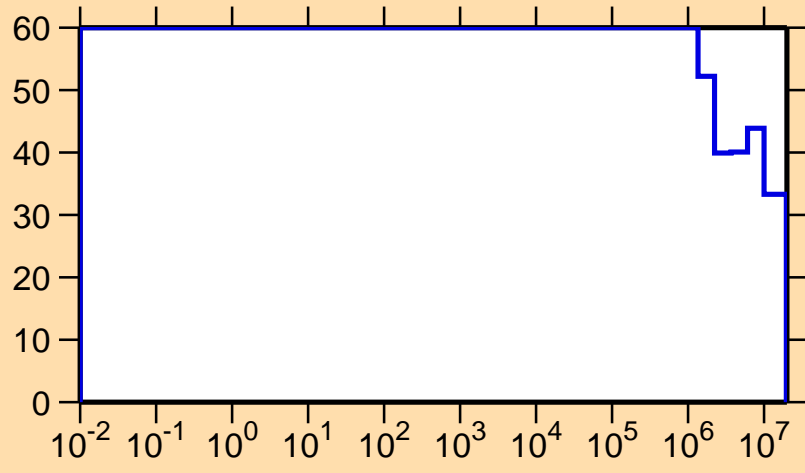
\Delta\sigma/\sigma vs. E for ^{200}\text{At}(n,p)
