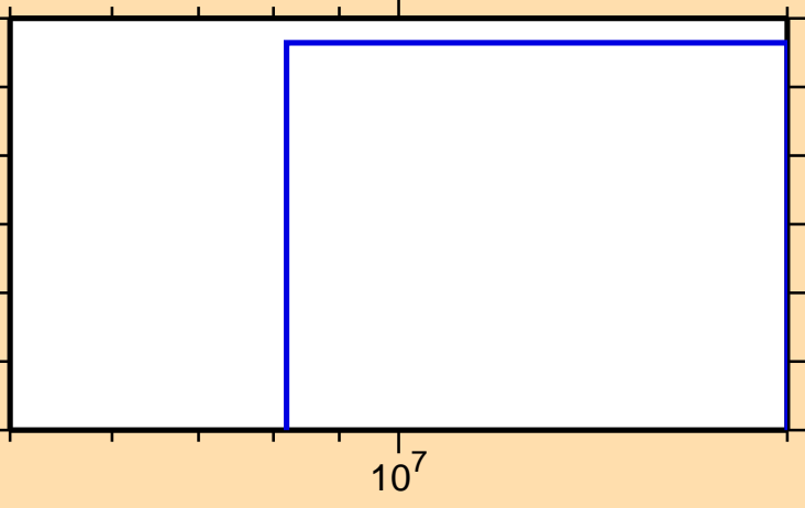
\sigma vs. E for ^{200}\text{At}(n,2n\alpha)
