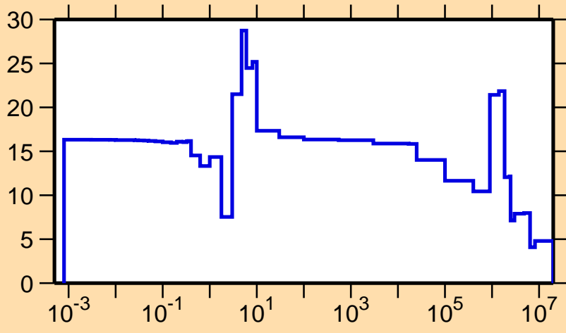
\Delta\sigma/\sigma vs. E for ^{200}\text{At}(n,el.)
