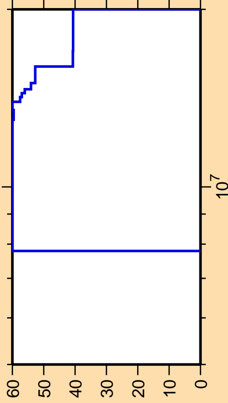
\Delta\sigma/\sigma vs. E for ^{200}\text{At}(n,2n)
