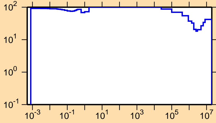
\Delta\sigma/\sigma vs. E for ^{200}\text{At}(n, \gamma)
