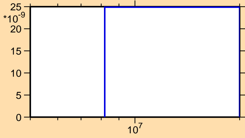
\sigma vs. E for ^{200}\text{At}(\text{mt } 45)
