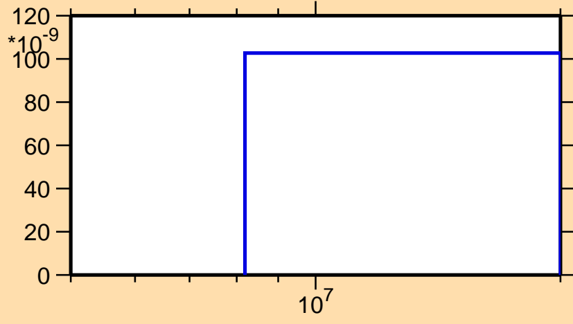
\sigma vs. E for ^{200}\text{At}(n,\text{nd})
