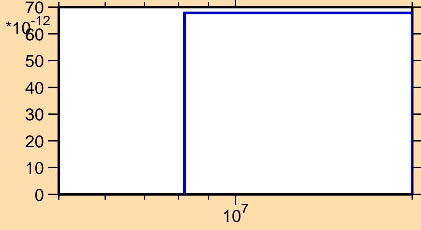
\sigma vs. E for ^{200}\text{At}(n,pt)
