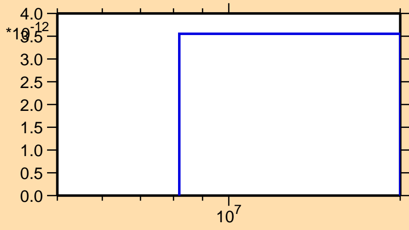
\sigma vs. E for ^{200}\text{At}(\text{mt } 34)
