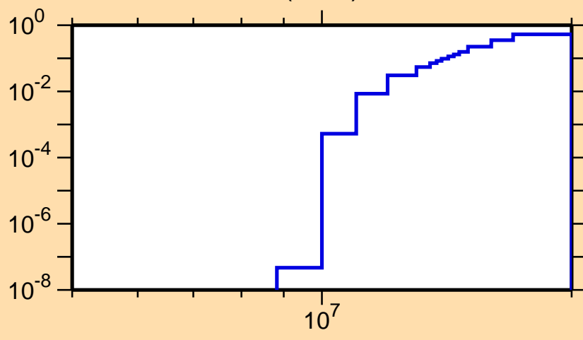
\sigma vs. E for ^{201}\text{At}(n,2n)
