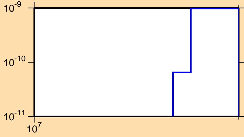
\sigma vs. E for ^{201}\text{At}(n,3n\alpha)
