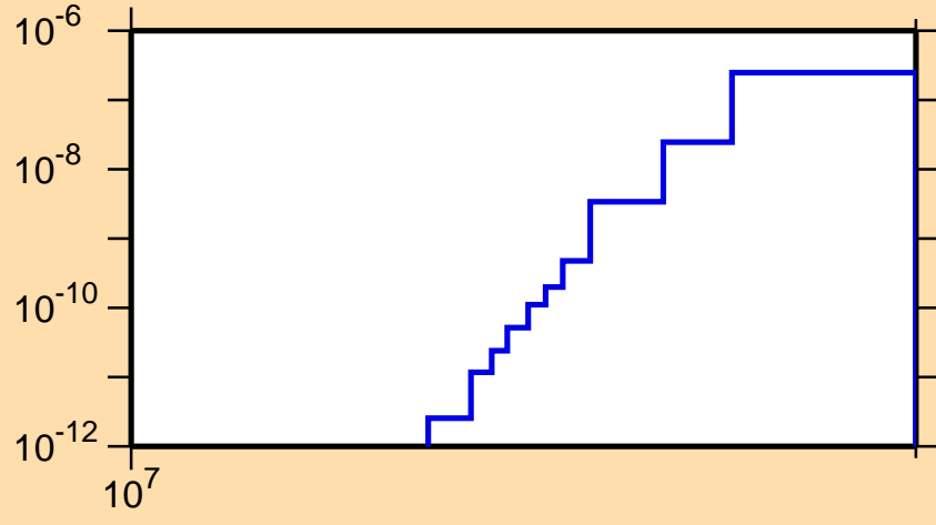
\sigma vs. E for ^{201}\text{At}(n,nd)
