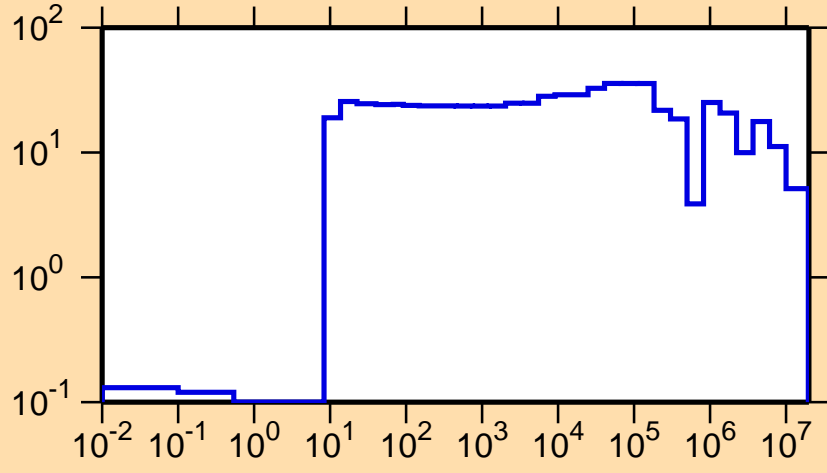
\Delta\sigma/\sigma vs. E for ^{201}\text{At}(n,el.)
