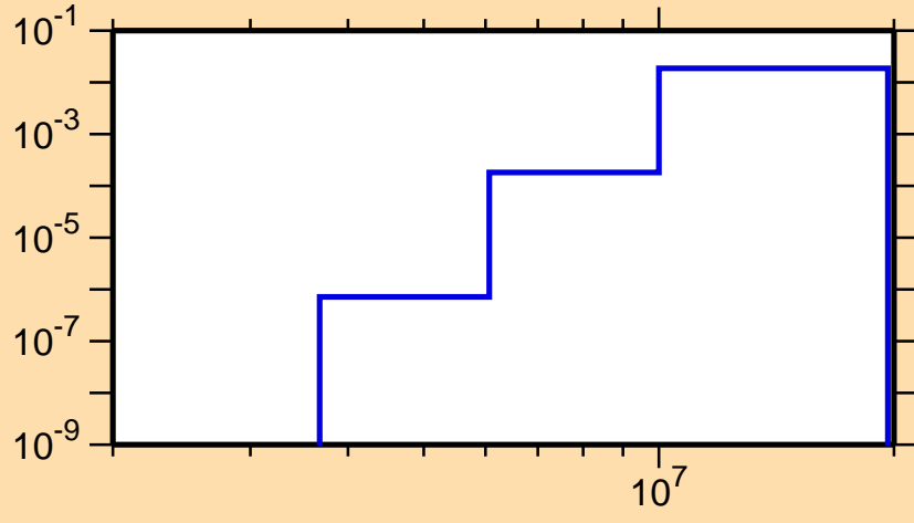
\sigma vs. E for ^{201}\text{At}(n,np)
