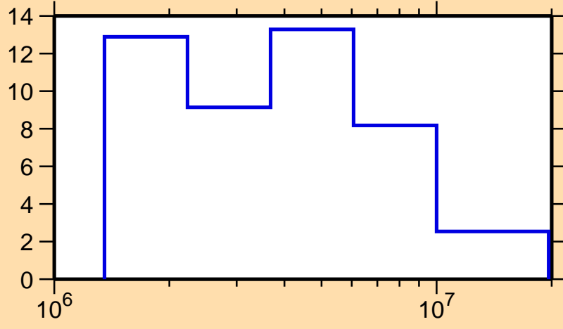
\Delta\sigma/\sigma vs. E for ^{201}\text{At}(n,tot.)
