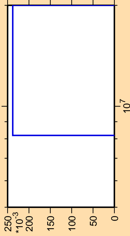
\Delta\sigma/\sigma vs. E for ^{201}\text{At}(\text{mt } 34)
