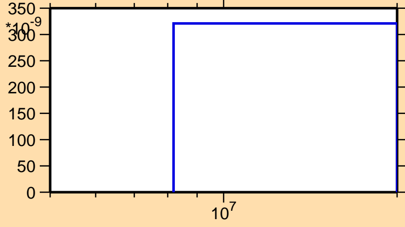
\sigma vs. E for ^{201}\text{At}(n,2np)
