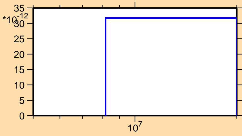
\sigma vs. E for ^{201}\text{At}(n,nt)
