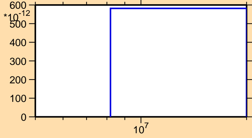
\sigma vs. E for ^{201}\text{At}(n,\text{pd})
