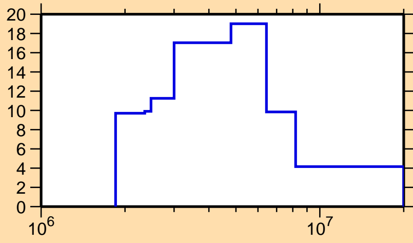
\Delta\sigma/\sigma vs. E for ^{201}\text{At}(n, el.)
