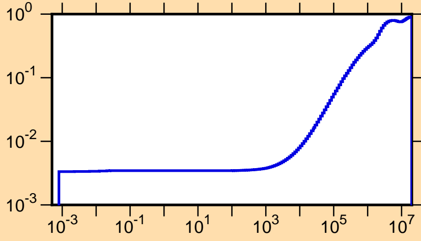
\mu vs. E for ^{202}\text{At}(\text{mt251})
