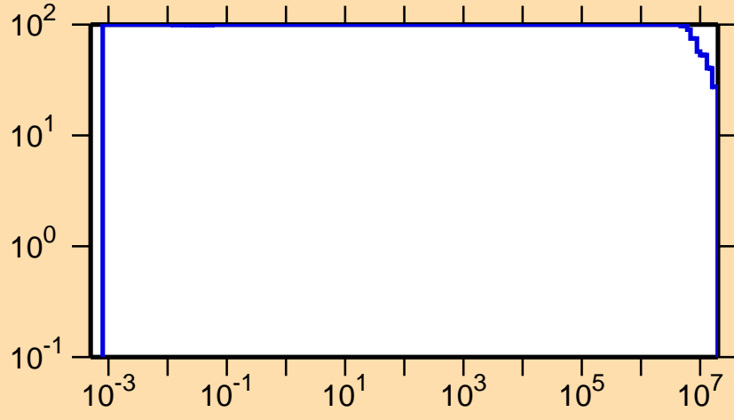
\Delta\sigma/\sigma vs. E for ^{202}\text{At}(n, p)
