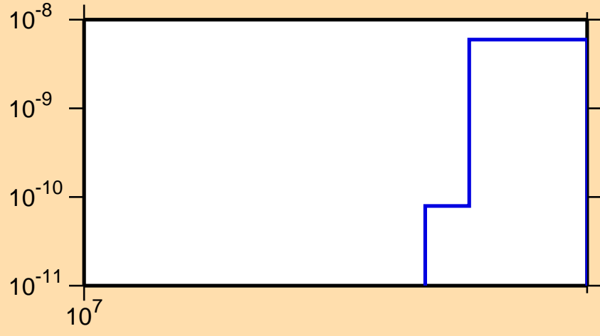
\sigma vs. E for ^{202}\text{At}(n,nt)
