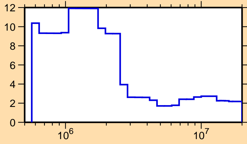
\Delta\sigma/\sigma vs. E for ^{202}\text{At}(n,\text{nonel.})
