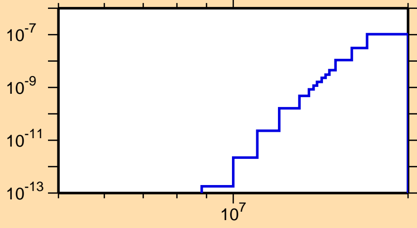
\sigma vs. E for ^{202}\text{At}(\text{mt } 45)
