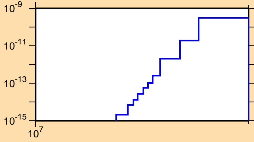
\sigma vs. E for ^{202}\text{At}(\text{mt } 34)
