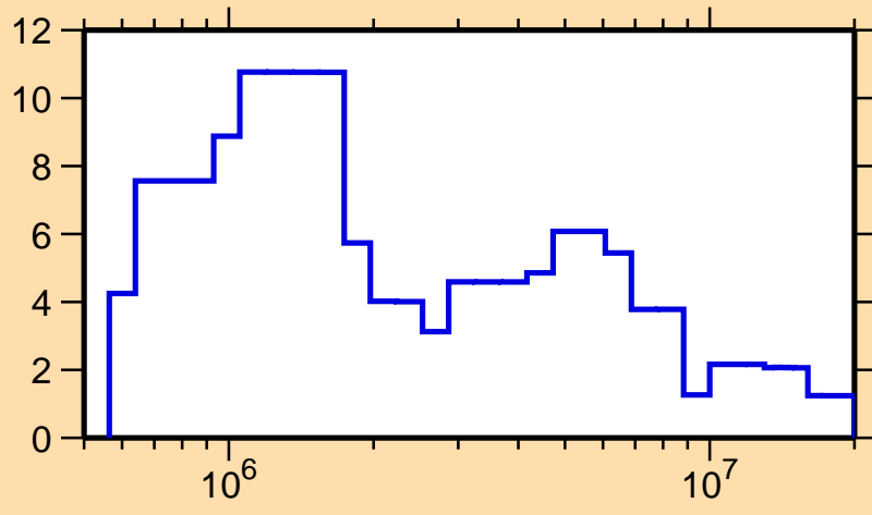
\Delta\sigma/\sigma vs. E for ^{202}\text{At}(n,\text{el.})
