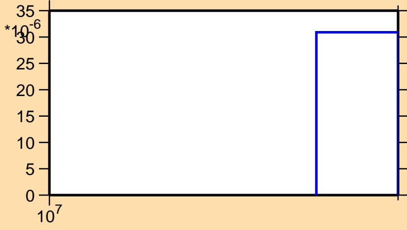
\sigma vs. E for ^{202}\text{At}(n,3n)
