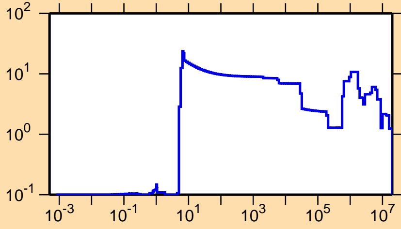
\Delta\sigma/\sigma vs. E for ^{202}\text{At}(n, \text{el.})
