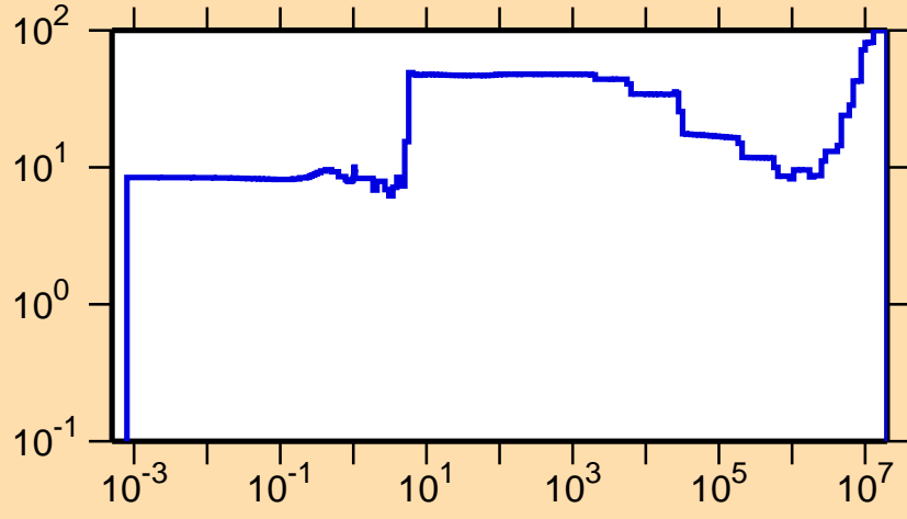
\Delta\sigma/\sigma vs. E for ^{202}\text{At}(n,\gamma)
