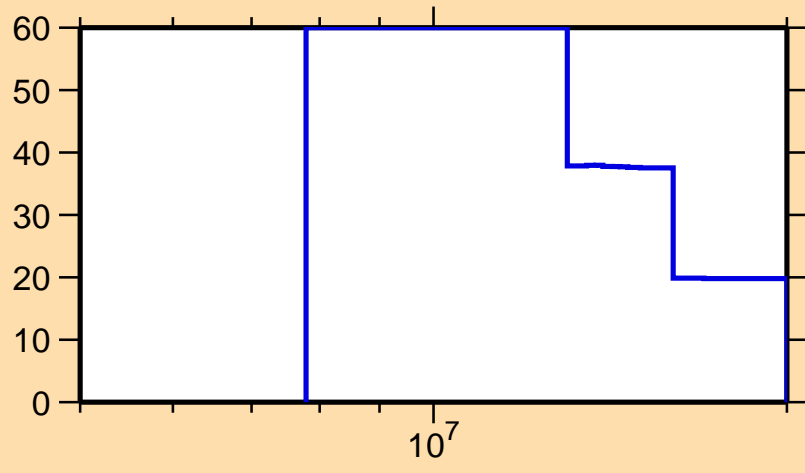
\Delta\sigma/\sigma vs. E for ^{202}\text{At}(n,2n)
