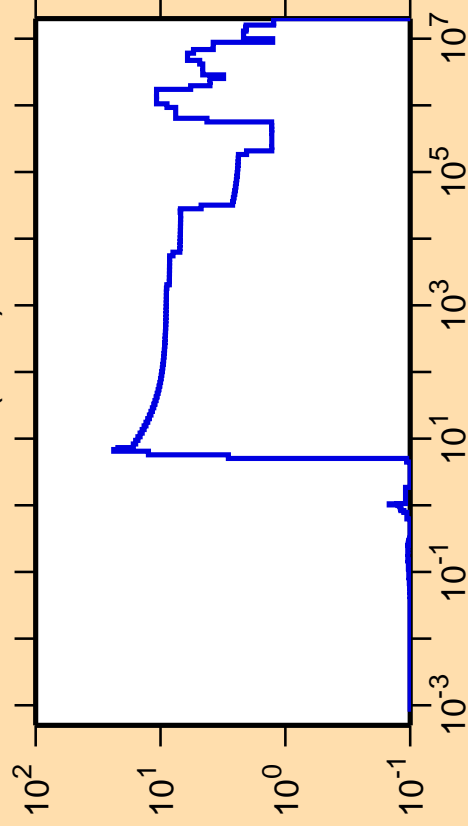
\Delta\sigma/\sigma vs. E for ^{202}\text{At}(n,\text{el.})
