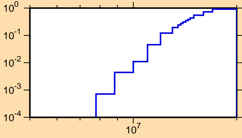
\sigma vs. E for ^{202}\text{At}(n,2n)
