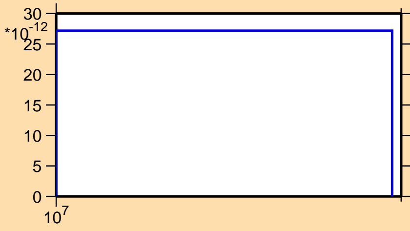
\sigma vs. E for ^{202}\text{At}(n,pt)
