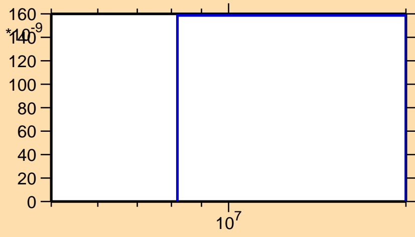
\sigma vs. E for ^{202}\text{At}(n,\text{nd})
