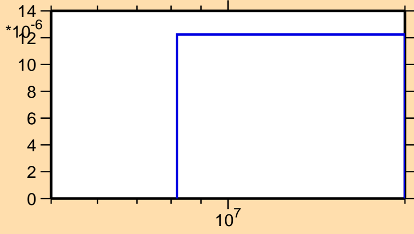
\sigma vs. E for ^{202}\text{At}(n,2np)
