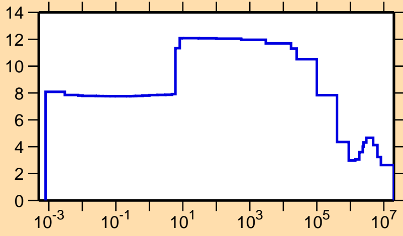
\sigma vs. E for ^{202}\text{At}(n,\text{el.})
