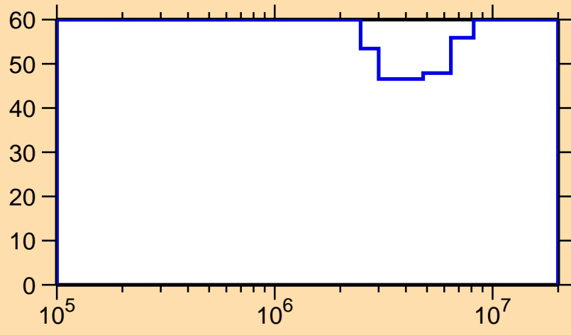
\Delta\sigma/\sigma vs. E for ^{202}\text{At}(n,n_1)
