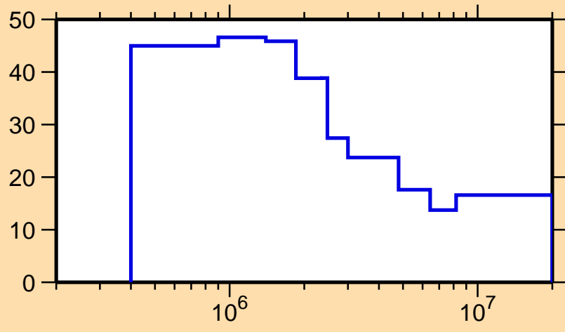
\Delta\sigma/\sigma vs. E for ^{202}\text{At}(n,n\text{cont.})
