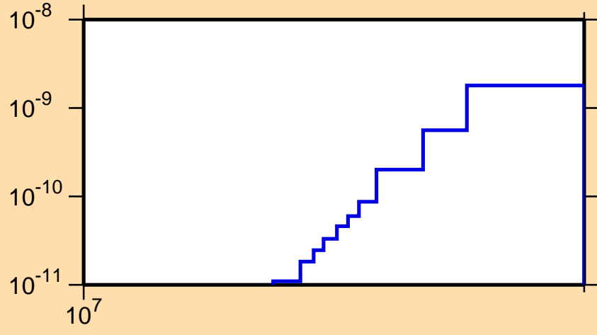
\sigma vs. E for ^{202}\text{At}(\text{mt117})
