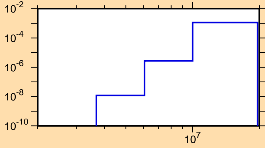
\sigma vs. E for ^{202}\text{At}(n,n\alpha)
