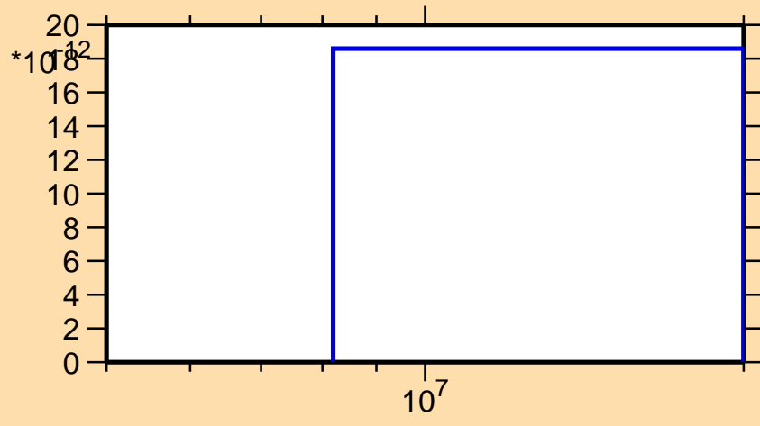
\sigma vs. E for ^{202}\text{At}(n,\text{pt})
