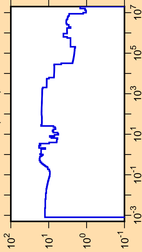
\Delta\sigma/\sigma vs. E for ^{203}\text{At}(n,\text{tot.})
