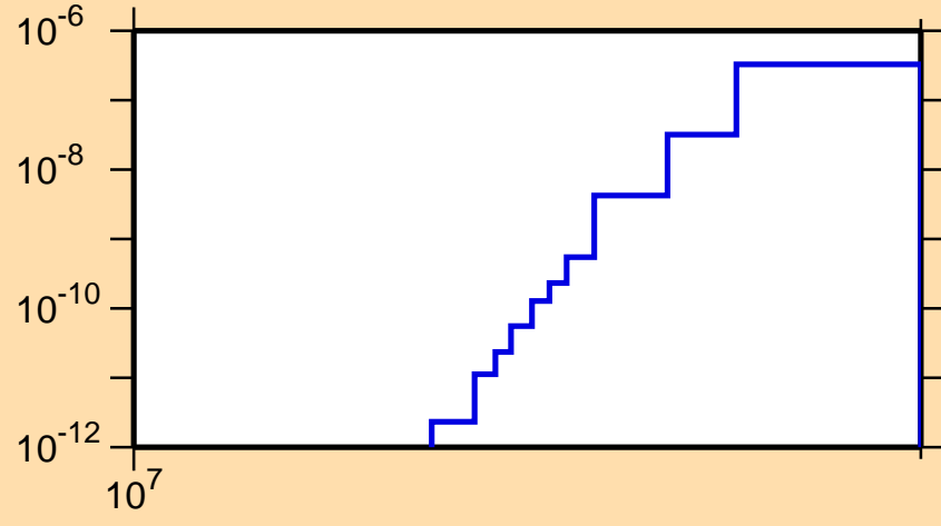
\sigma vs. E for ^{203}\text{At}(n,\text{nd})
