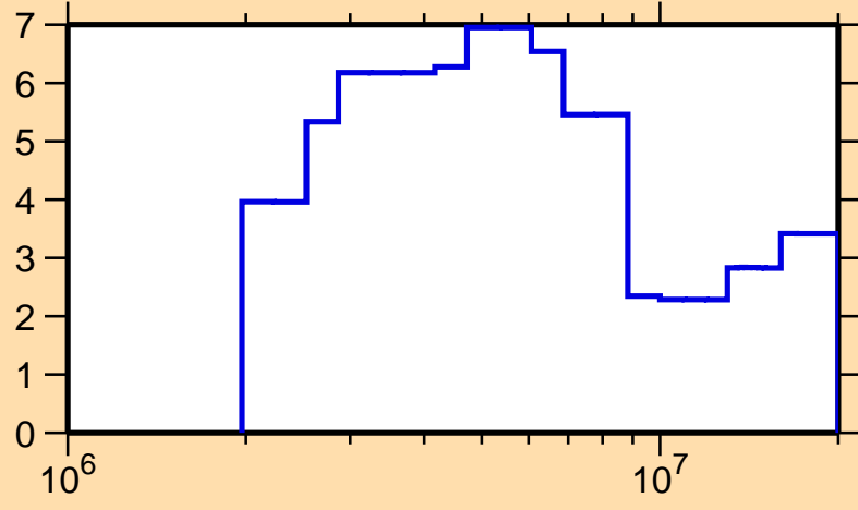
\Delta\sigma/\sigma vs. E for ^{203}\text{At}(n, el.)
