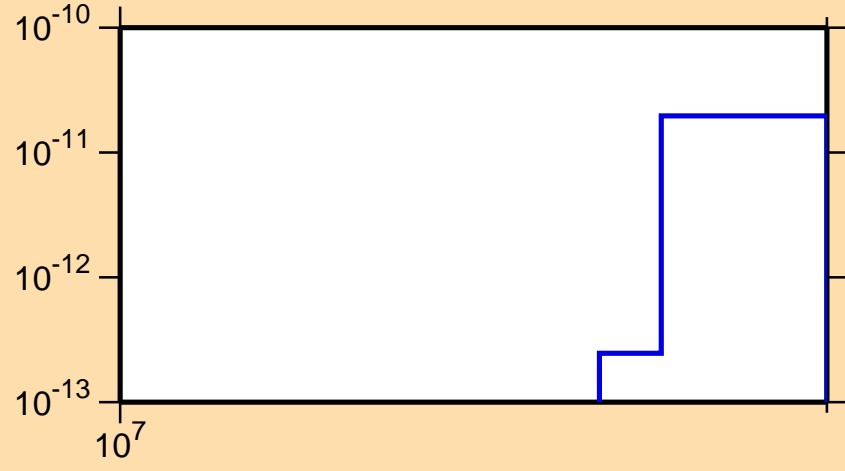
\sigma vs. E for ^{203}\text{At}(n,pt)
