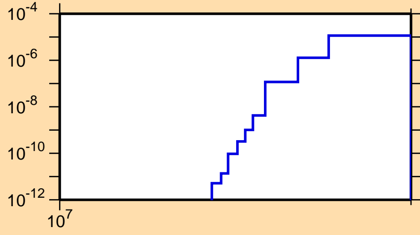
\sigma vs. E for ^{203}\text{At}(n,2np)
