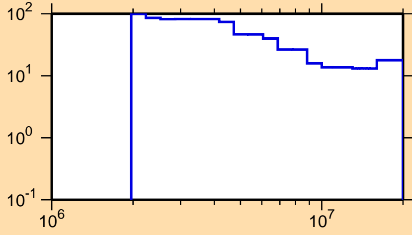
\Delta\sigma/\sigma vs. E for ^{203}\text{At}(n,n\text{cont.})
