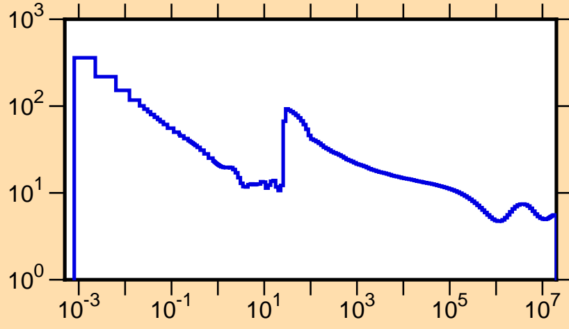
\sigma vs. E for ^{203}\text{At}(n,\text{tot.})
