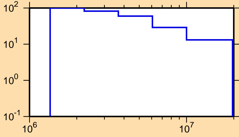
\Delta\sigma/\sigma vs. E for ^{203}\text{At}(n,ncont.)
