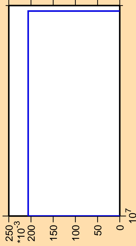
\Delta\sigma/\sigma vs. E for ^{203}\text{At}(\text{mt } 34)
