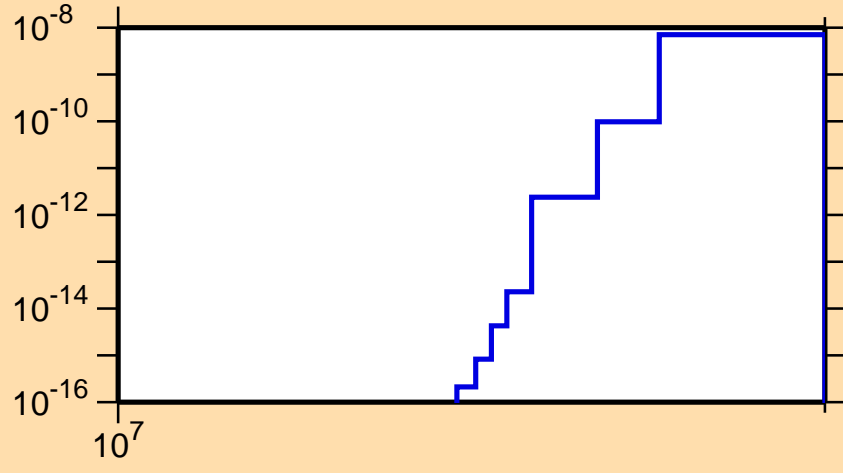
\sigma vs. E for ^{204}\text{At}(n,nt)
