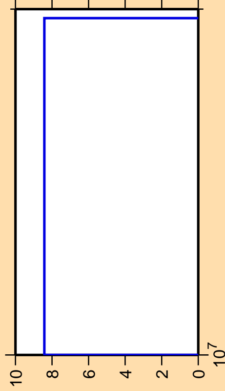
\Delta\sigma/\sigma vs. E for ^{204}\text{At}(n,\text{pt})
