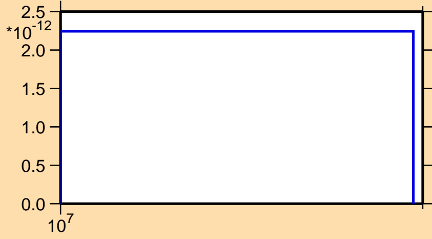
\sigma vs. E for ^{204}\text{At}(n,\text{pt})
