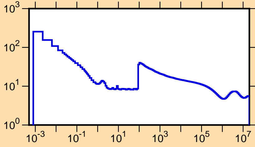
\sigma vs. E for ^{205}\text{At}(n,\text{tot.})
