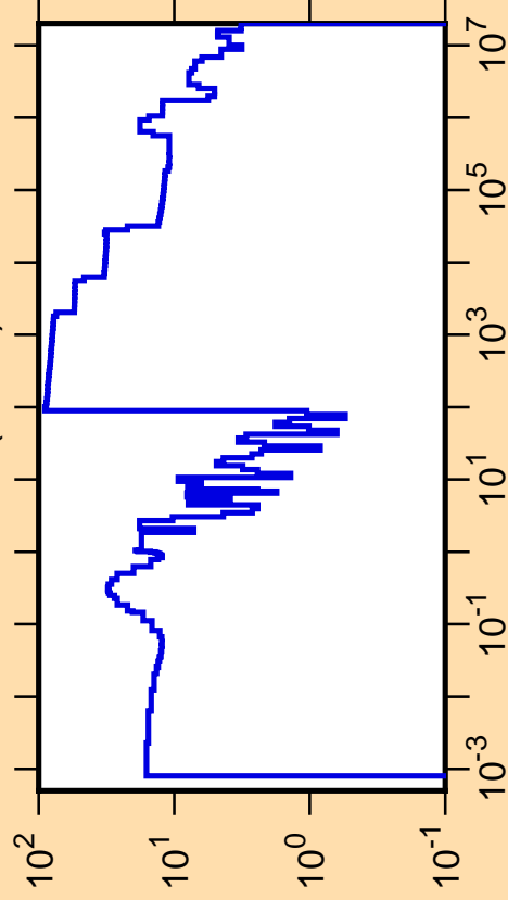
\Delta\sigma/\sigma vs. E for ^{205}\text{At}(n,\text{tot.})
