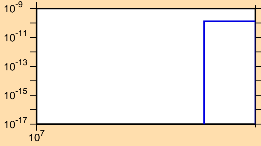
\sigma vs. E for ^{205}\text{At}(n,3n\alpha)
