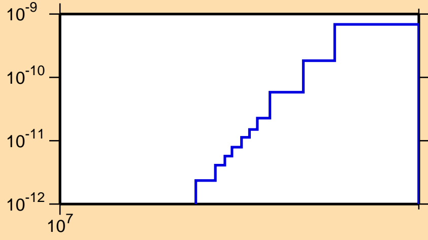
\sigma vs. E for ^{205}\text{At}(\text{mt117})
