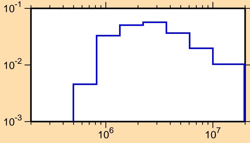
\sigma vs. E for ^{205}\text{At}(n,n_3)
