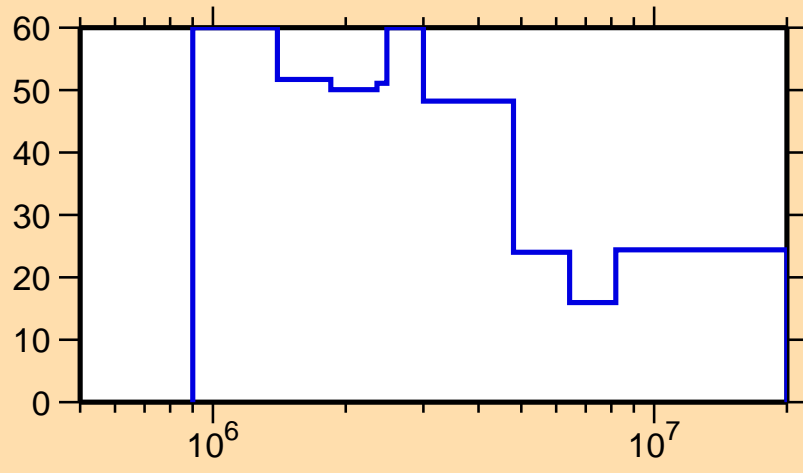
\Delta\sigma/\sigma vs. E for ^{205}\text{At}(n,n\text{cont.})
