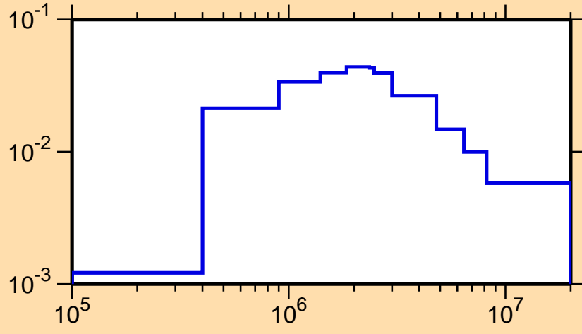
\sigma vs. E for ^{205}\text{At}(n,n_1)
