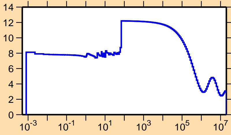
\sigma vs. E for ^{206}\text{At}(n,\text{el.})
