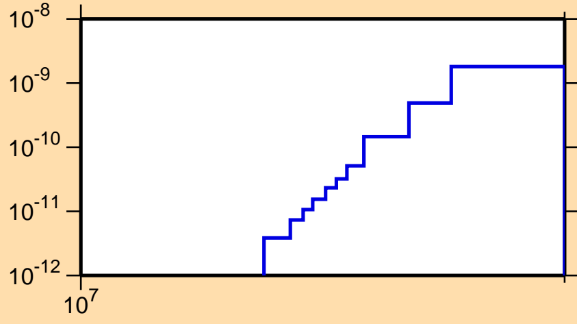
\sigma vs. E for ^{206}\text{At}(\text{mt117})
