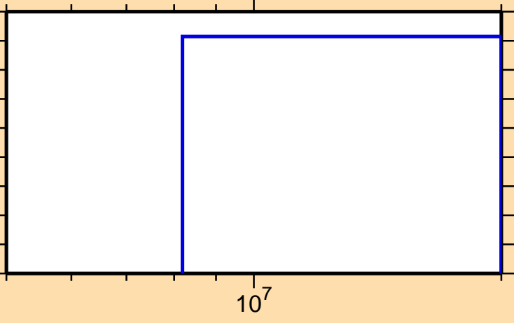
\sigma vs. E for ^{206}\text{At}(n,2np)
