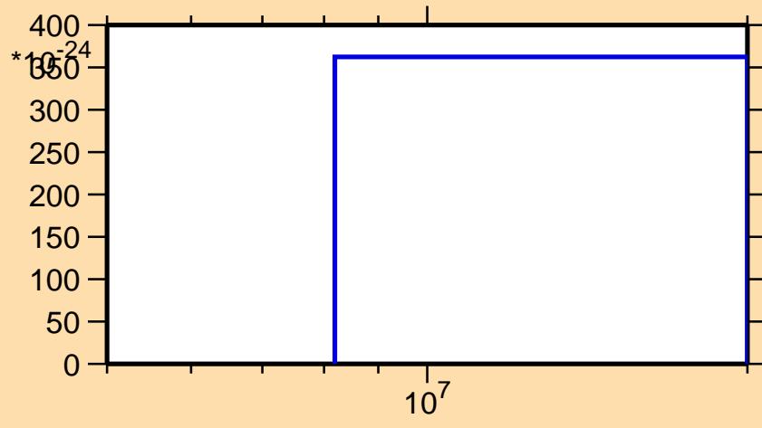
\sigma vs. E for ^{206}\text{At}(\text{mt } 42)
