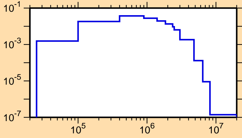
\sigma vs. E for ^{206}\text{At}(n,n_2)
