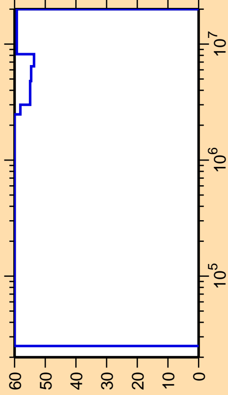
\Delta\sigma/\sigma vs. E for ^{206}\text{At}(n,n_2)
