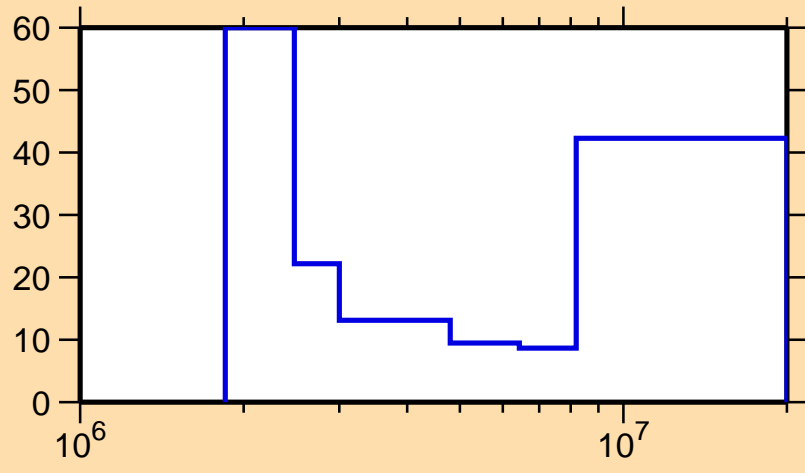
\Delta\sigma/\sigma vs. E for ^{207}\text{At}(n,ncont.)
