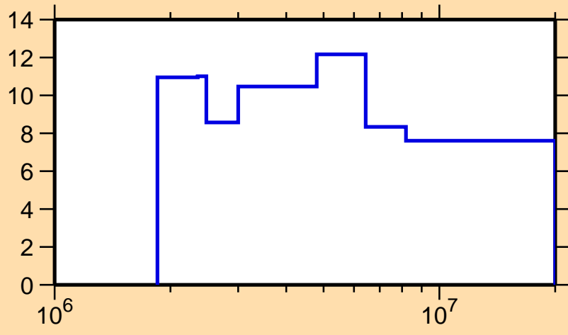
\Delta\sigma/\sigma vs. E for ^{207}\text{At}(n, el.)
