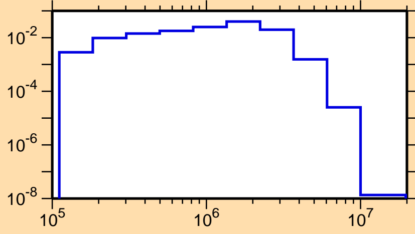
\sigma vs. E for ^{208}\text{At}(n,n_4)
