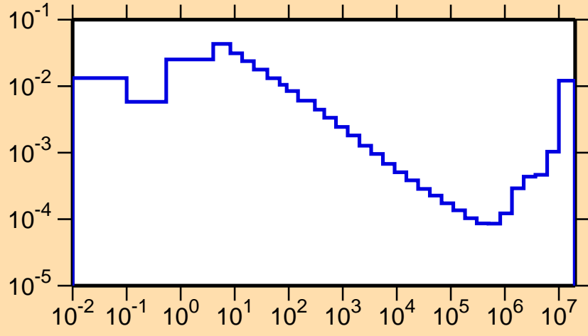
\sigma vs. E for ^{208}\text{At}(n,\alpha)
