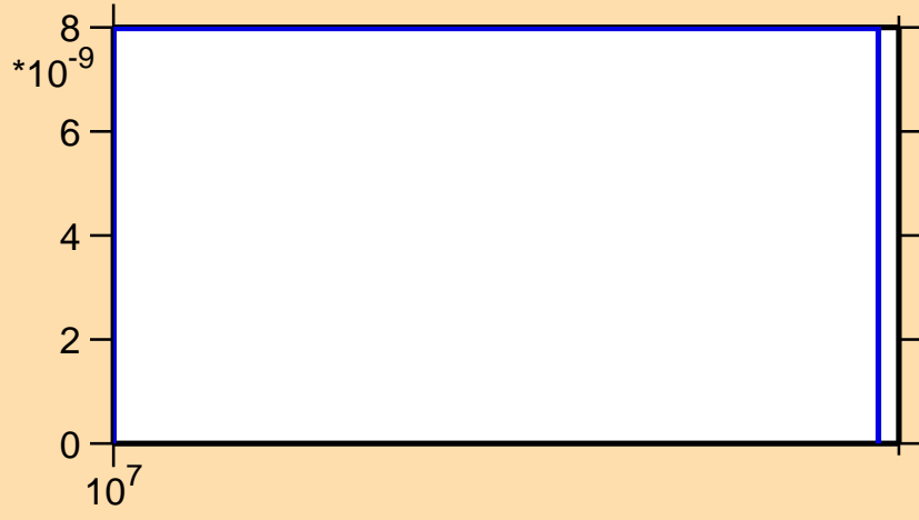
\sigma vs. E for ^{208}\text{At}(n,nt)
