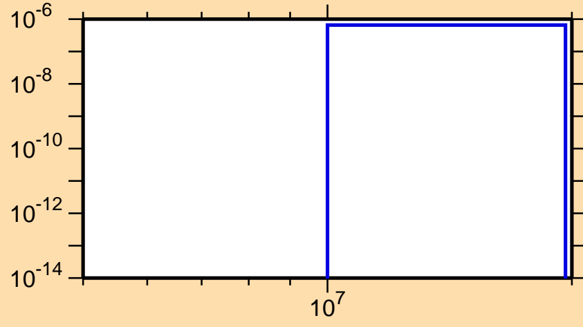
\sigma vs. E for ^{208}\text{At}(n,\text{nd})
