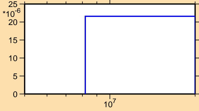
\sigma vs. E for ^{208}\text{At}(n,2np)
