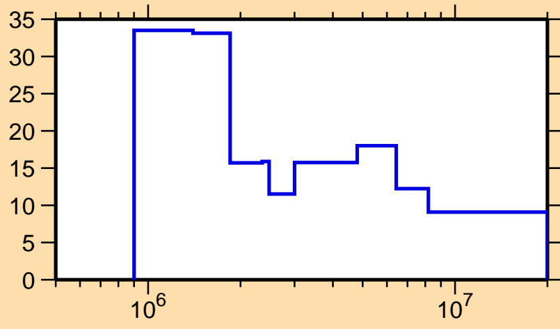
\Delta\sigma/\sigma vs. E for ^{208}\text{At}(n, el.)
