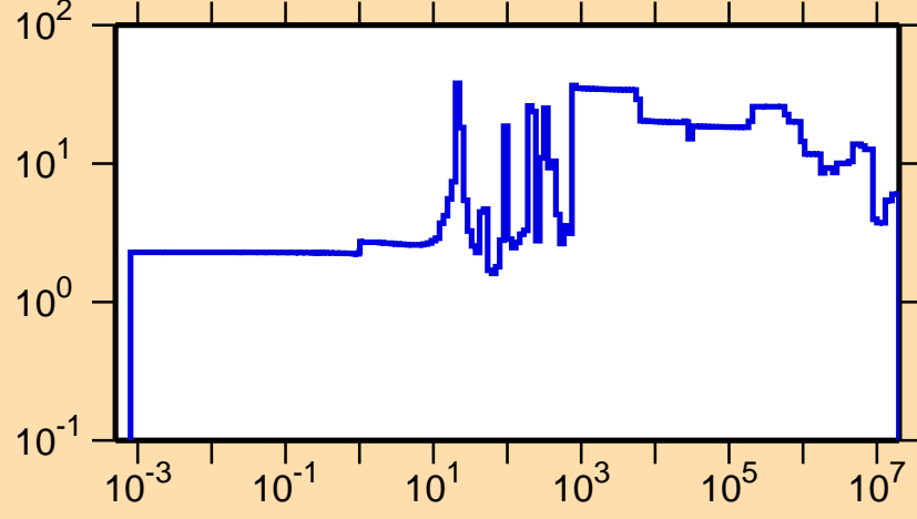
\Delta\sigma/\sigma vs. E for ^{209}\text{At}(n,el.)
