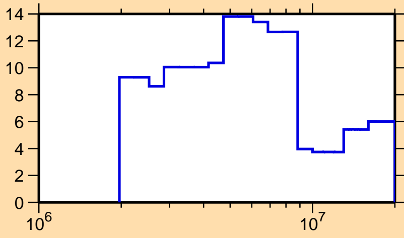
\Delta\sigma/\sigma vs. E for ^{209}\text{At}(n, el.)
