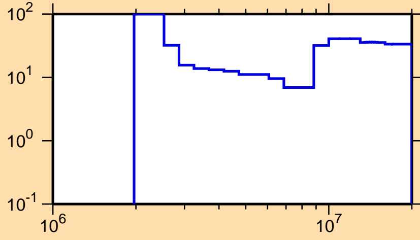
\Delta\sigma/\sigma vs. E for ^{209}\text{At}(n,ncont.)
