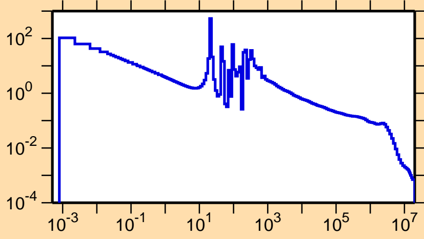
\sigma vs. E for ^{209}\text{At}(n,\gamma)
