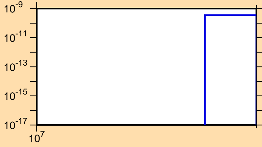
\sigma vs. E for ^{209}\text{At}(n,3n\alpha)
