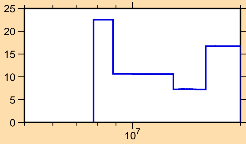
\Delta\sigma/\sigma vs. E for ^{209}\text{At}(n,2n)
