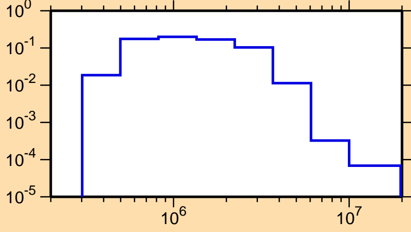
\sigma vs. E for ^{209}\text{At}(n,n_1)
