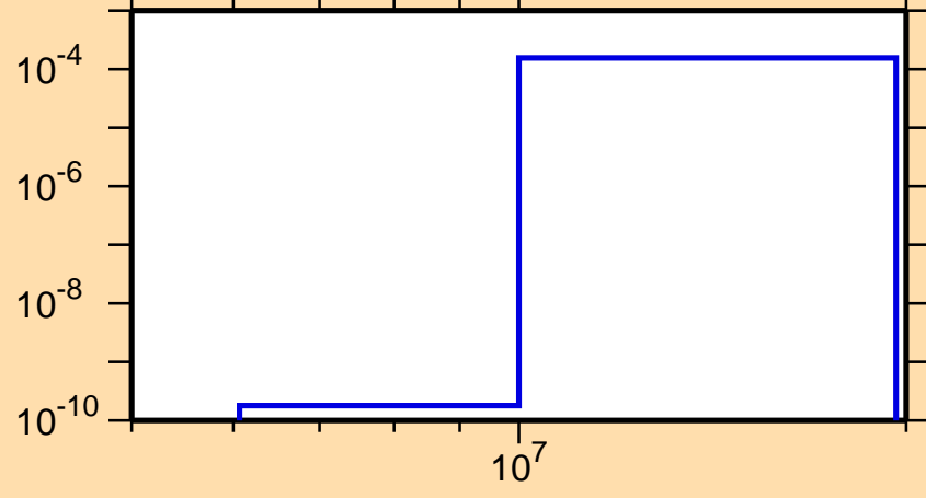
\sigma vs. E for ^{209}\text{At}(n,t)
