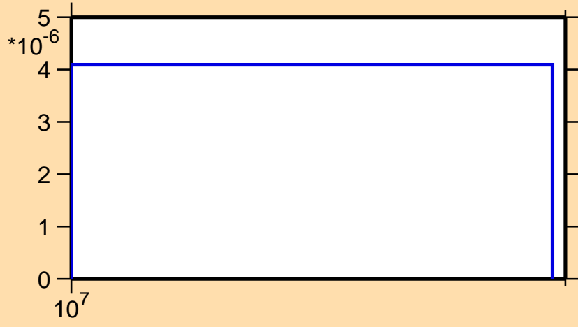
\sigma vs. E for ^{209}\text{At}(n,2np)
