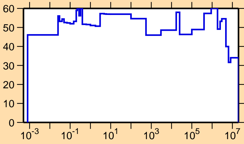
\Delta\sigma/\sigma vs. E for ^{209}\text{At}(n,p)
