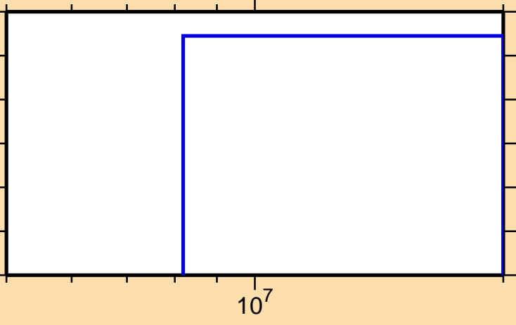
\sigma vs. E for ^{209}\text{At}(n,nt)
