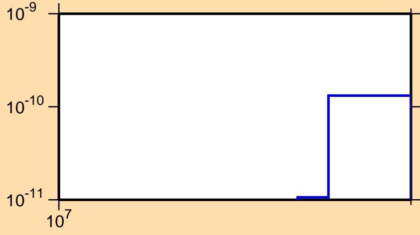
\sigma vs. E for ^{210}\text{At}(n,\text{pd})
