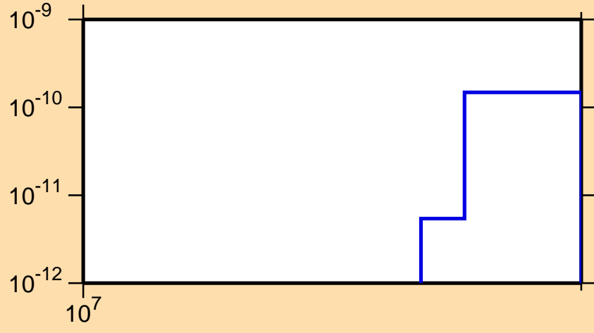
\sigma vs. E for ^{210}\text{At}(n,pt)
