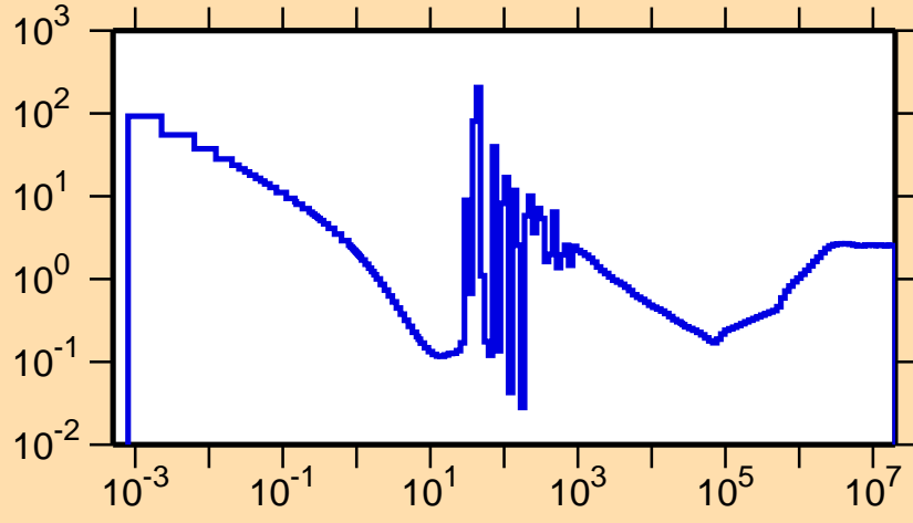
\sigma vs. E for ^{210}\text{At}(n,\text{nonel.})
