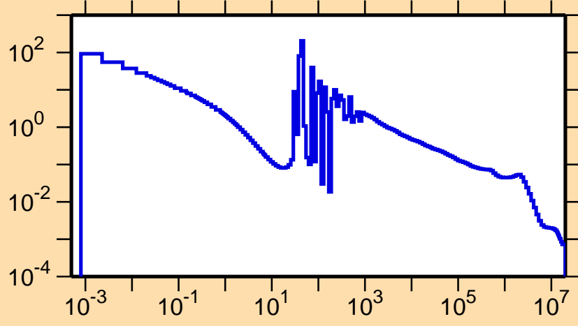
\sigma vs. E for ^{210}\text{At}(n,\gamma)
