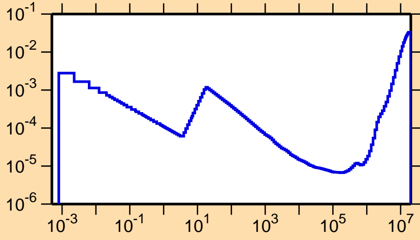
\sigma vs. E for ^{210}\text{At}(n,p)
