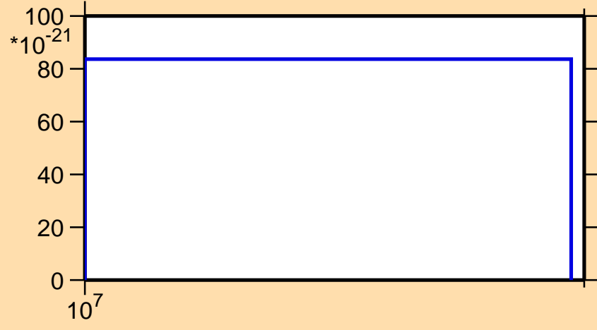
\sigma vs. E for ^{210}\text{At} (mt 42)
