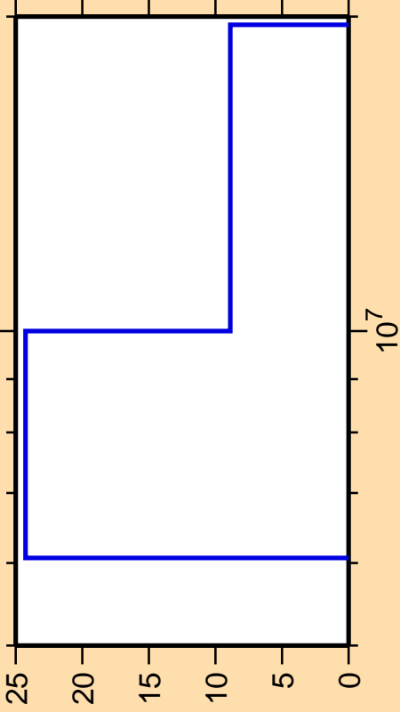
\Delta\sigma/\sigma vs. E for ^{210}\text{At}(n,2n)
