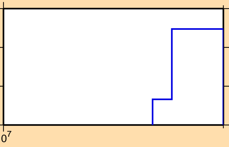
\sigma vs. E for ^{211}\text{At}(n,pt)
