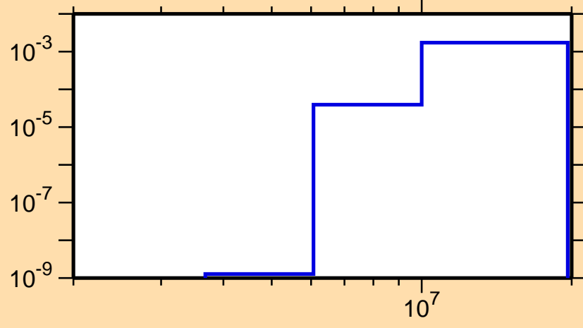
\sigma vs. E for ^{211}\text{At}(n,np)
