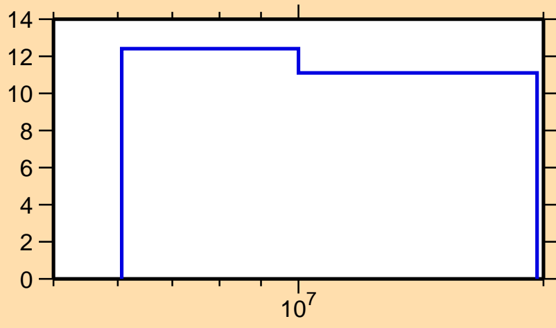
\Delta\sigma/\sigma vs. E for ^{211}\text{At}(n,2n)
