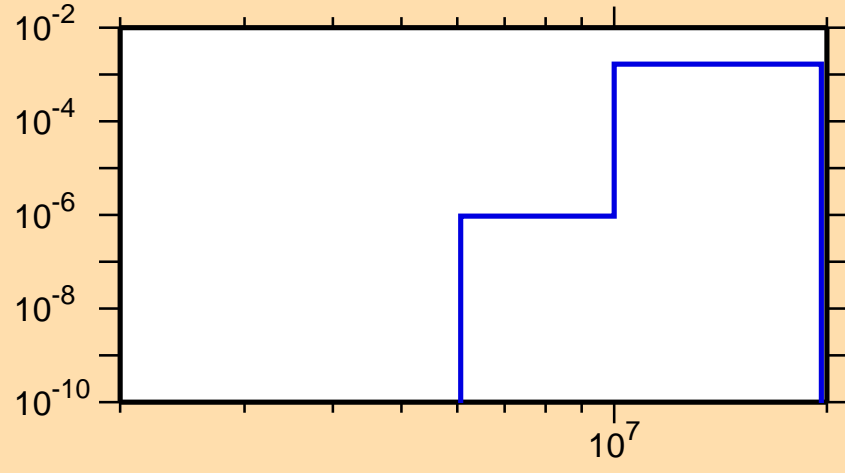
\sigma vs. E for ^{211}\text{At}(n,d)
