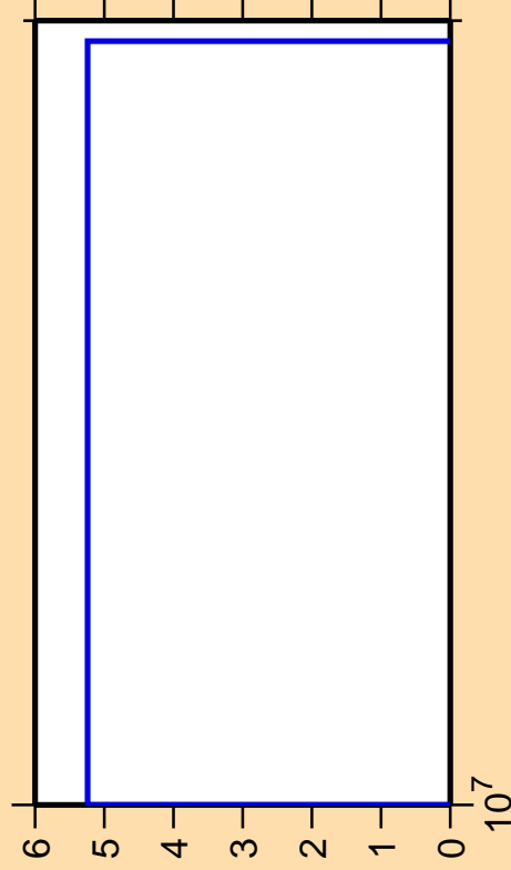
\Delta\sigma/\sigma vs. E for ^{211}\text{At}(n,\text{pd})
