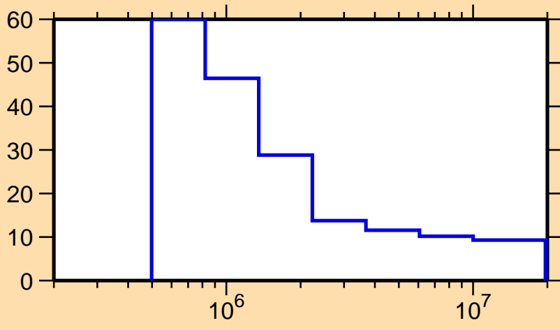
\Delta\sigma/\sigma vs. E for ^{211}\text{At}(n,\text{nonel.})
