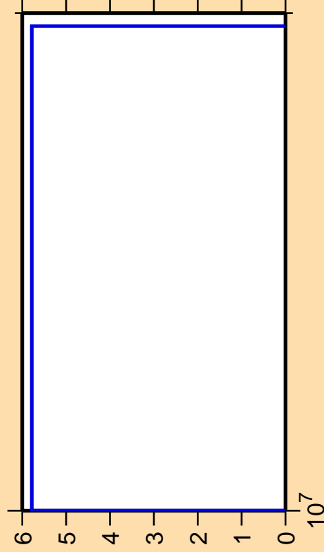
\Delta\sigma/\sigma vs. E for ^{211}\text{At}(n,3n\alpha)
