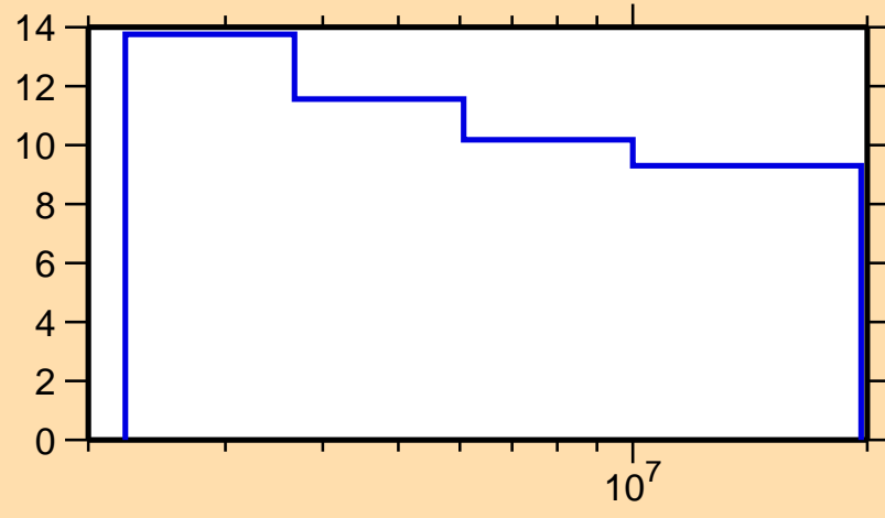
\Delta\sigma/\sigma vs. E for ^{211}\text{At}(n,n\text{onel.})
