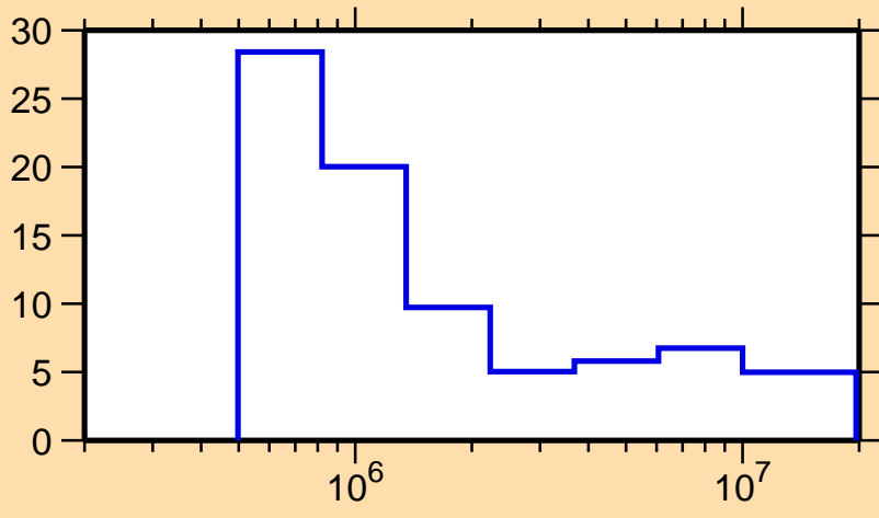
\Delta\sigma/\sigma vs. E for ^{211}\text{At}(n,\text{tot.})
