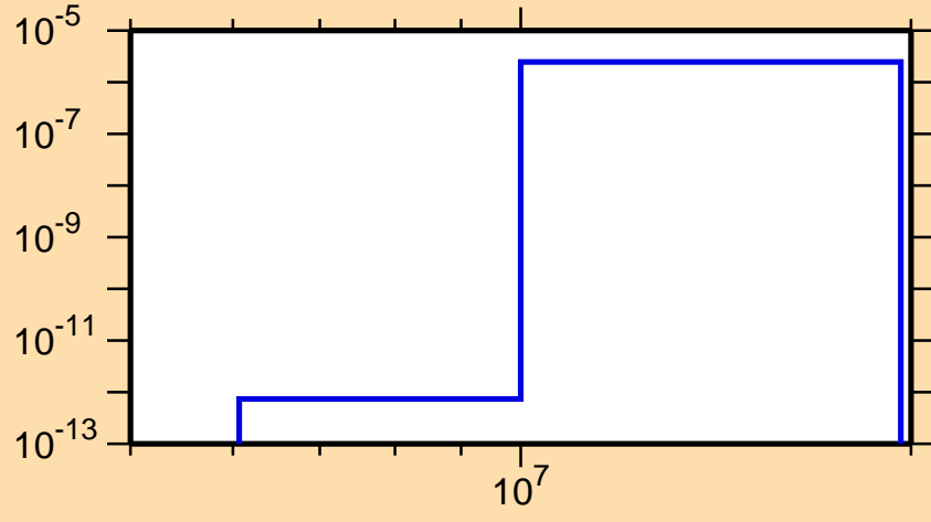
\sigma vs. E for ^{211}\text{At}(n,2n\alpha)
