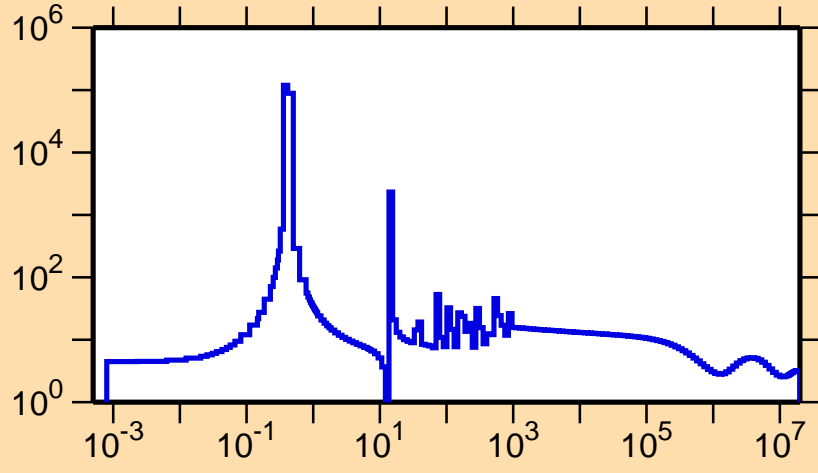
\sigma vs. E for ^{218}\text{At}(n,\text{el.})
