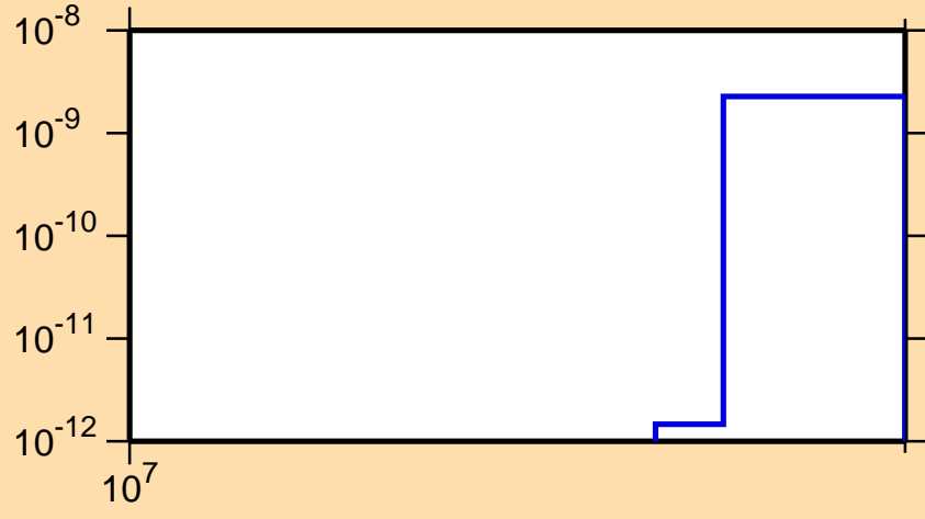
\sigma vs. E for ^{218}\text{At}(\text{mt } 11)
