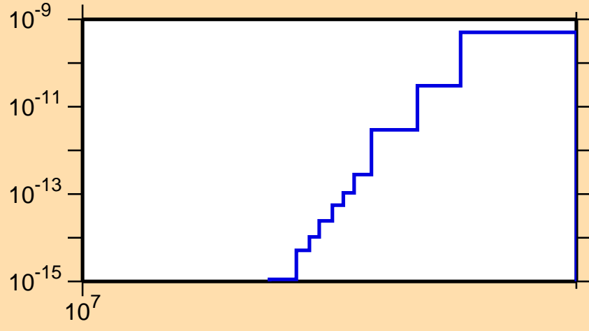
\sigma vs. E for ^{218}\text{At}(n,\text{He3})
