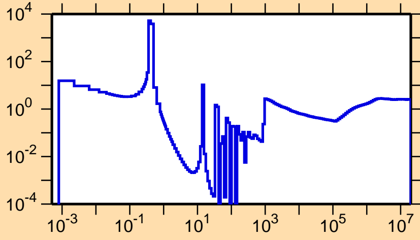
\sigma vs. E for ^{218}\text{At}(n,\text{nonel.})
